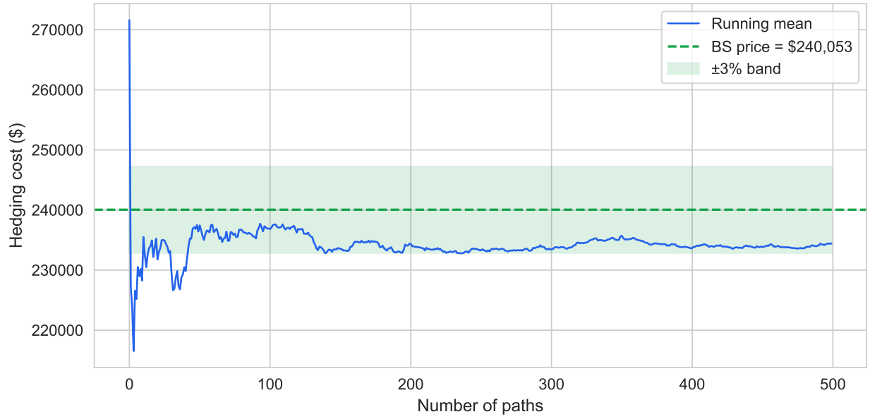
Figure 6.1: Running mean of hedging cost across 500 seeded GBM paths converges to the Black-Scholes price. Shaded band: \pm 3\% of the BS price. Source: synthetic GBM, seed 20260519.
