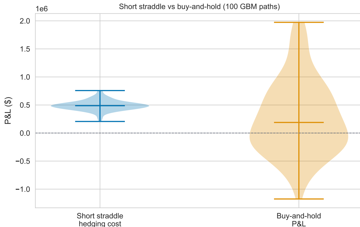
Figure 6.7: Short straddle hedging cost distribution vs. buy-and-hold P&L across 100 seeded GBM paths ( S = 49 , K = 50 , \sigma = 20\% , T = 20 wks). The straddle collects premium from both legs at inception; the hedging cost distribution is wider than a single-leg position because both ITM and OTM settlement branches contribute. Source: synthetic GBM, base seed 20260519 + offset 1000 (seeds 20261519–20261618).
