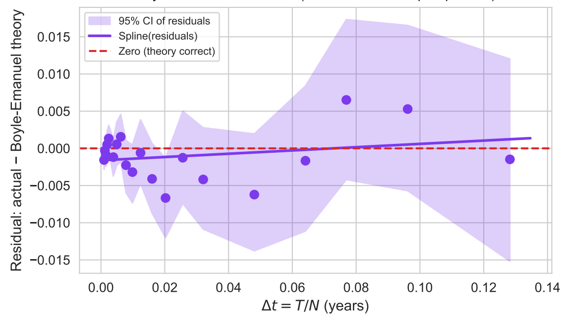
Boyle-Emanuel residuals (zero in band \Leftrightarrow spec passes)
