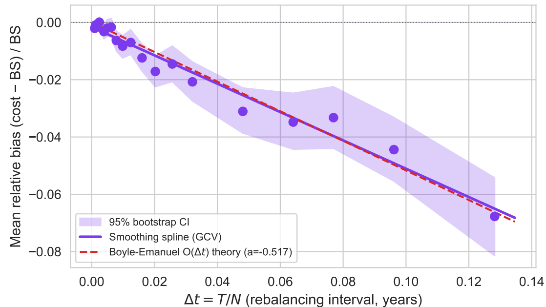
Boyle-Emanuel O(\Delta t) bias: PASS, theory within CI
