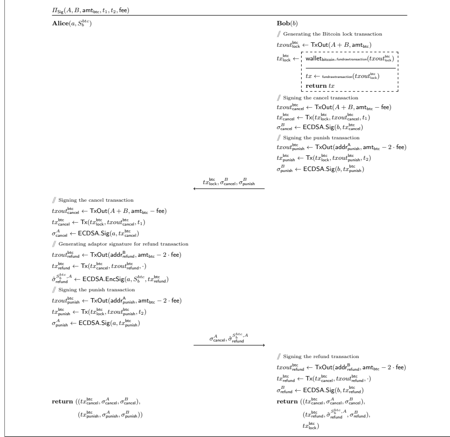
Fig. 3. Signing protocol. Both parties must verify the signatures received, but this is left out for clarity.
