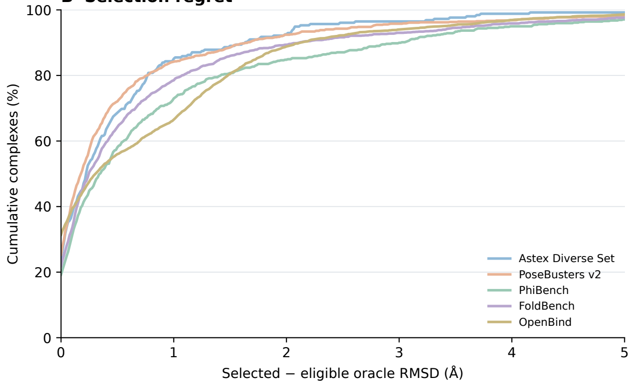
B Selection regret
