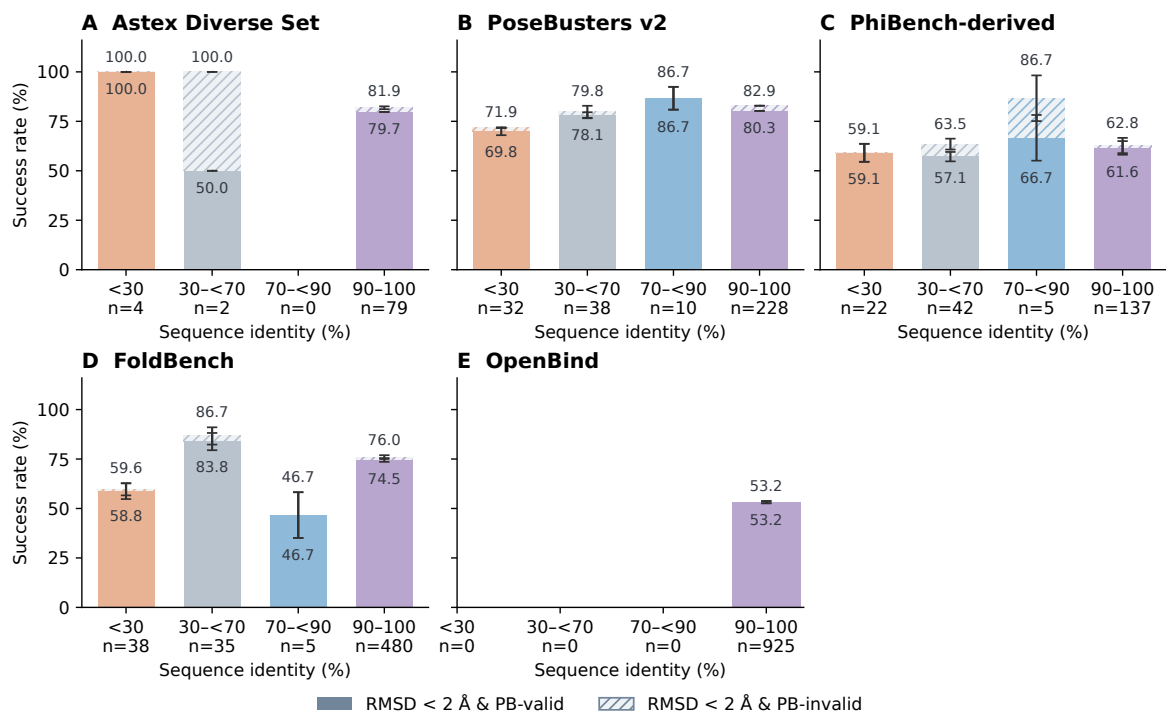
Figure S8: Docking performance by training-set sequence identity. Strata use maximum query-normalized binding-chain identity to the docking-training set. Solid bars show RMSD–PoseBusters success, coloured by identity stratum (the dark legend patch denotes solid fill); hatching extends to RMSD-only success. Bars and whiskers show three-repeat means and sample SD; labels give stratum sizes, including empty and sparse groups.
