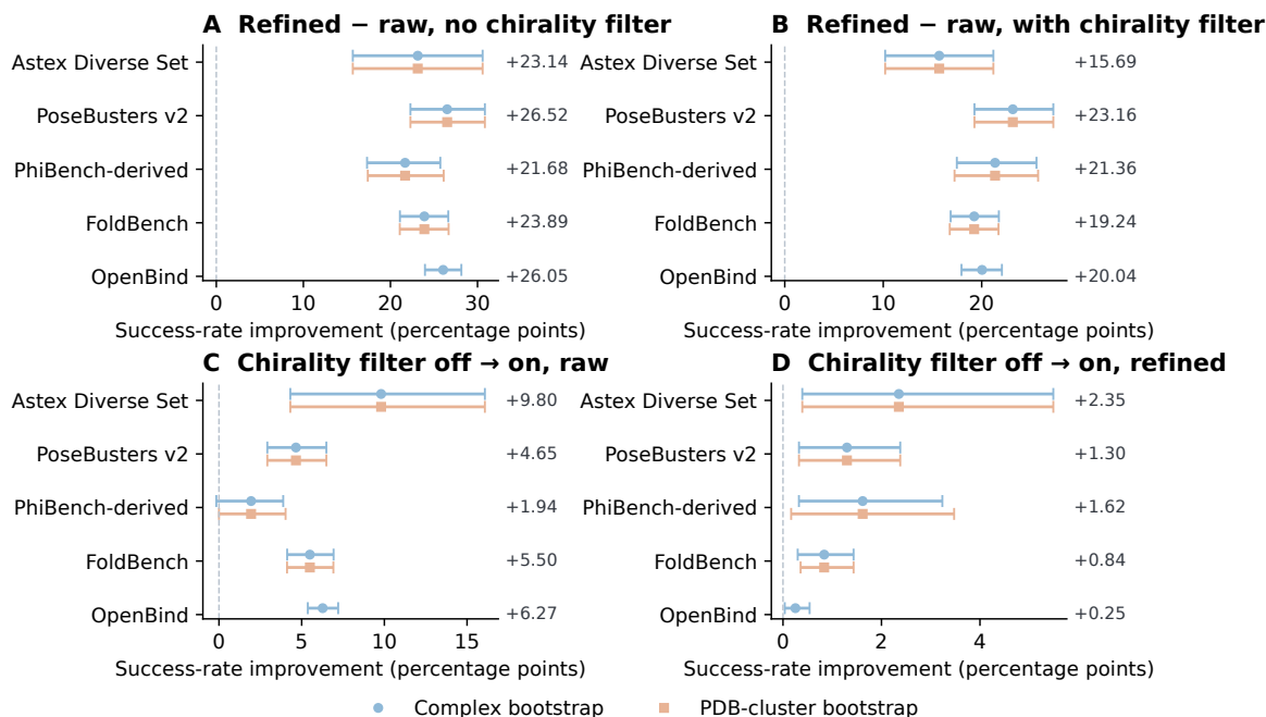
Figure S9: Paired changes in docking success with refinement and chirality filtering. EFF-Dock results compare refined versus raw candidates with and without the chirality filter and filter off versus on at each stage. The endpoint is RMSD < 2 Å and PoseBusters success. Per-complex paired differences are averaged across seeds before 2,000-draw percentile bootstrapping. Whiskers show complex and exact-PDB-cluster 95% intervals; OpenBind lacks a cluster interval.
