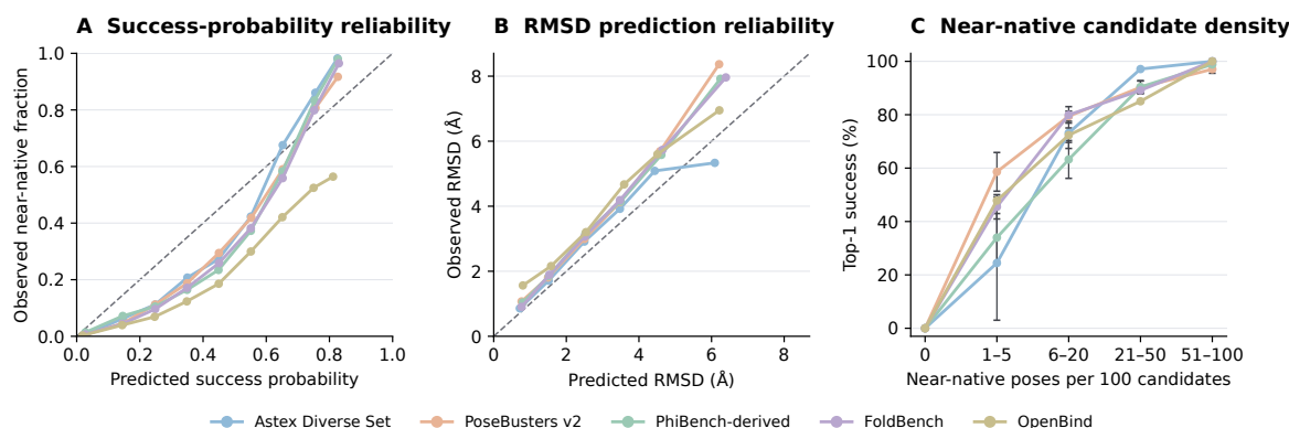
Figure S12: Reliability of saved confidence predictions and candidate-density dependence. EFF-Dock refined candidates are pooled across three repeats. (A) Empirical near-native fraction versus the saved success-head probability. (B) Mean observed versus predicted RMSD in fixed predicted-RMSD bins. No recalibration is fitted. (C) Primary chirality-filtered top-1 RMSD success versus the number of near-native candidates in the 100-pose bank; whiskers show sample SD across three repeats. Candidate observations within complexes are correlated, and the production selector uses predicted RMSD rather than the auxiliary probability head.
