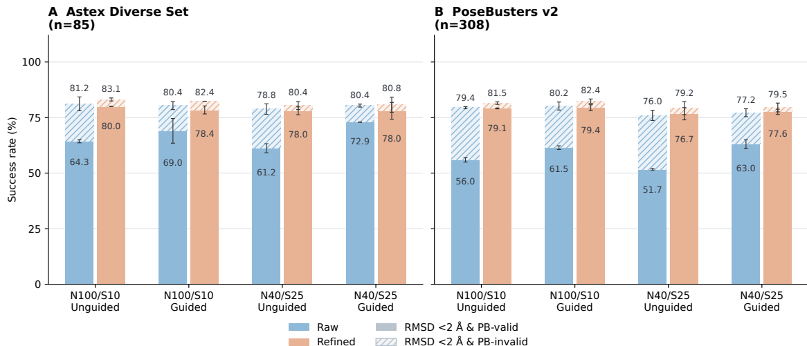
Figure S19: Guidance and candidate allocation at a fixed learned pose-step count. (A) Astex Diverse Set (85 complexes) and (B) PoseBusters v2 (308 complexes). N denotes poses and S integration steps. Each 100-pose/ten-step (N100/S10) or 40-pose/25-step (N40/S25) condition uses 1,000 learned pose-steps, with unguided generation or normalized energy guidance of strength \eta = 2 . Raw and refined banks use the input-chirality-filtered minimum-predicted-RMSD selector, with an unfiltered fallback. Solid segments show RMSD and PoseBusters success; hatched extensions show RMSD-successful but PB-invalid outcomes. Bars and whiskers show the mean and sample SD over three inference seeds. Guided and unguided initial draws are paired within each budget; the two budgets are separately executed. Equal pose-step counts are not equal-runtime comparisons.
