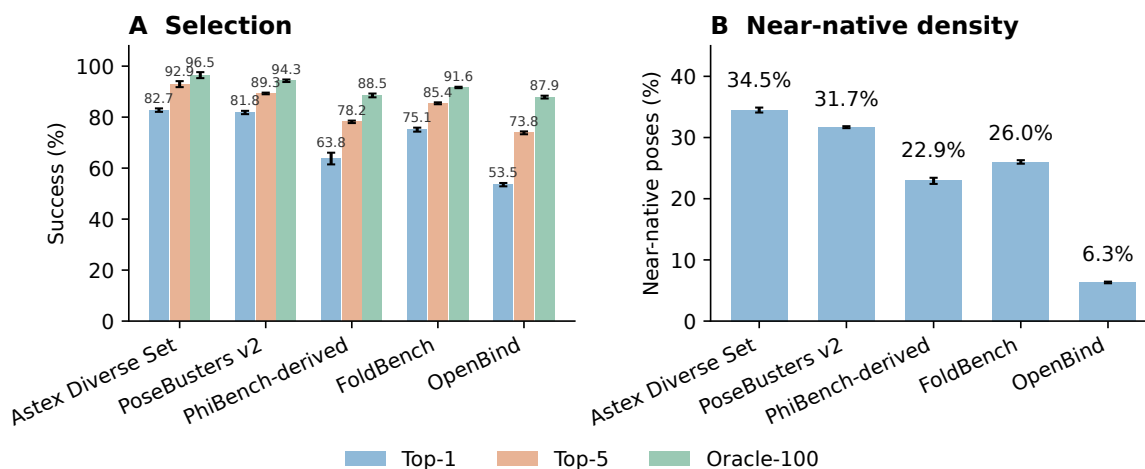
Figure S10: Confidence selection and near-native candidate density. (A) Unfiltered confidence top-1, top-5, and oracle-100 RMSD success for refined unguided banks; the primary chirality-filtered top-1 values are given in Fig. S13. (B) Fraction of individual refined candidates with RMSD < 2 Å. Bars show mean ± sample SD across three repeats. Panel A is measured per complex, whereas panel B is measured per candidate.
