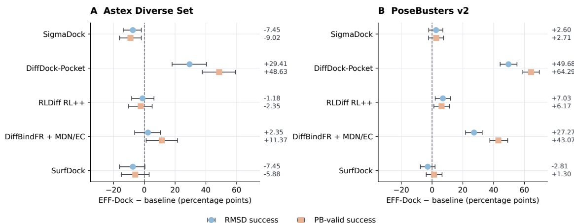
Figure S14: Paired uncertainty relative to locally executed baselines. EFF-Dock minus baseline percentage-point differences are shown for RMSD success and same-selected-pose RMSD–PoseBusters success (legend: PB-valid success) on (A) Astex Diverse Set and (B) PoseBusters v2. Intervals are 2,000-draw percentile 95% paired bootstrap intervals over exact PDB-accession groups; every retained complex has a distinct accession in these cohorts. Literature-only rows are excluded. Positive values favor EFF-Dock, but differing budgets and native selectors prevent an equal-compute superiority claim.
