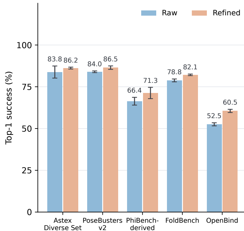
B Top-1 given an RMSD-successful candidate
