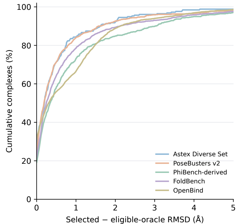
C Regret within the effective eligible set
