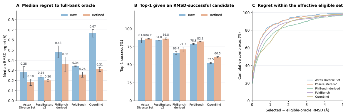
Figure S18: Selection regret and conditional top-1 success. EFF-Dock results use the primary chirality-filtered confidence selector. (A) Median selected-minus-full-bank-oracle RMSD regret for raw and refined banks. (B) Selected top-1 RMSD success among complexes whose full bank contains an RMSD-successful candidate. Losses in A and B can include chirality-eligibility exclusions. (C) Cumulative refined selected-pose RMSD regret relative to the minimum RMSD within the same effective eligible set, including the unfiltered fallback when no candidate passes the mask. The corresponding outcome partition is shown in main Fig. 5C. Reference RMSD is used only for retrospective analysis. Bars show three-repeat means and sample SD.
