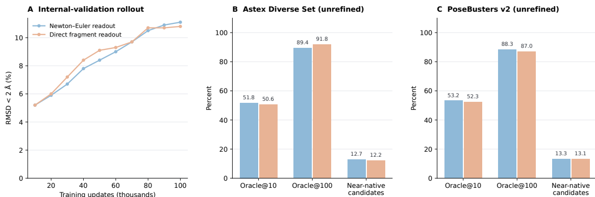
Figure S21: Matched readout ablation. Two docking models trained from scratch for 100,000 updates with a global batch of 16 complexes differ only in the output head: the Newton–Euler least-squares readout of atom vectors or a direct fragment readout. (A) Internal-validation rollout success (single sample, 20 steps, 1,076 complexes) every 10,000 updates using the EMA weights. (B,C) Unrefined 100-pose, ten-step banks on Astex Diverse Set and PoseBusters v2 at the terminal checkpoint: RMSD < 2 Å oracle coverage among the first 10 and all 100 generated candidates and the mean fraction of near-native candidates. One training seed per arm; no refinement or confidence ranking.
