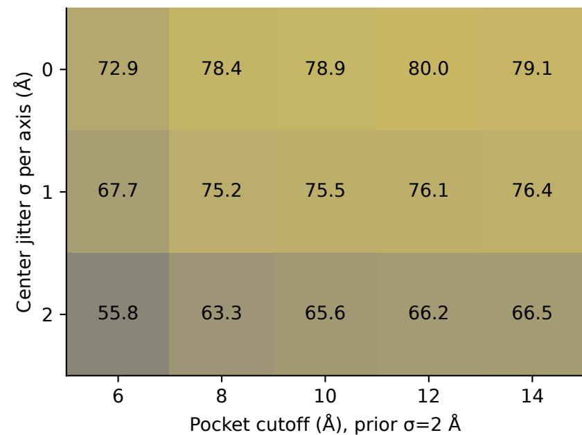
PoseBusters
