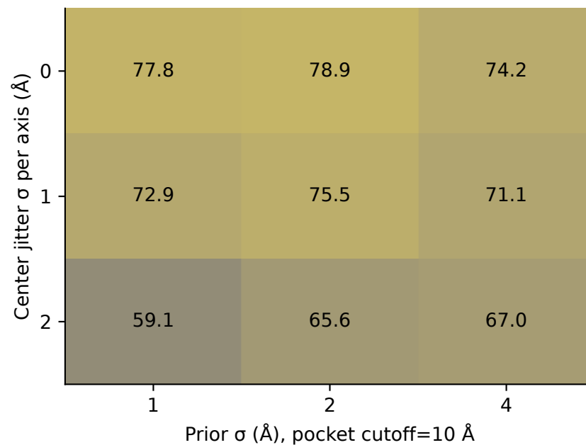
PoseBusters
