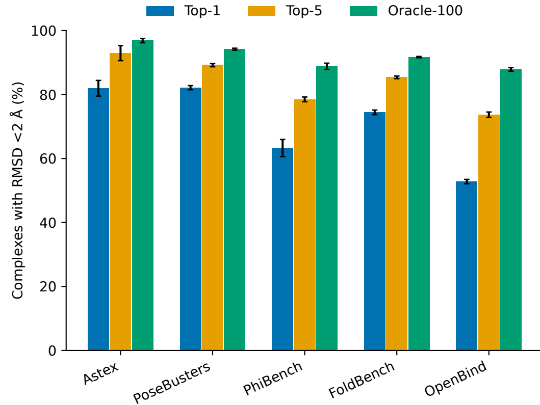
Confidence selection versus candidate coverage
