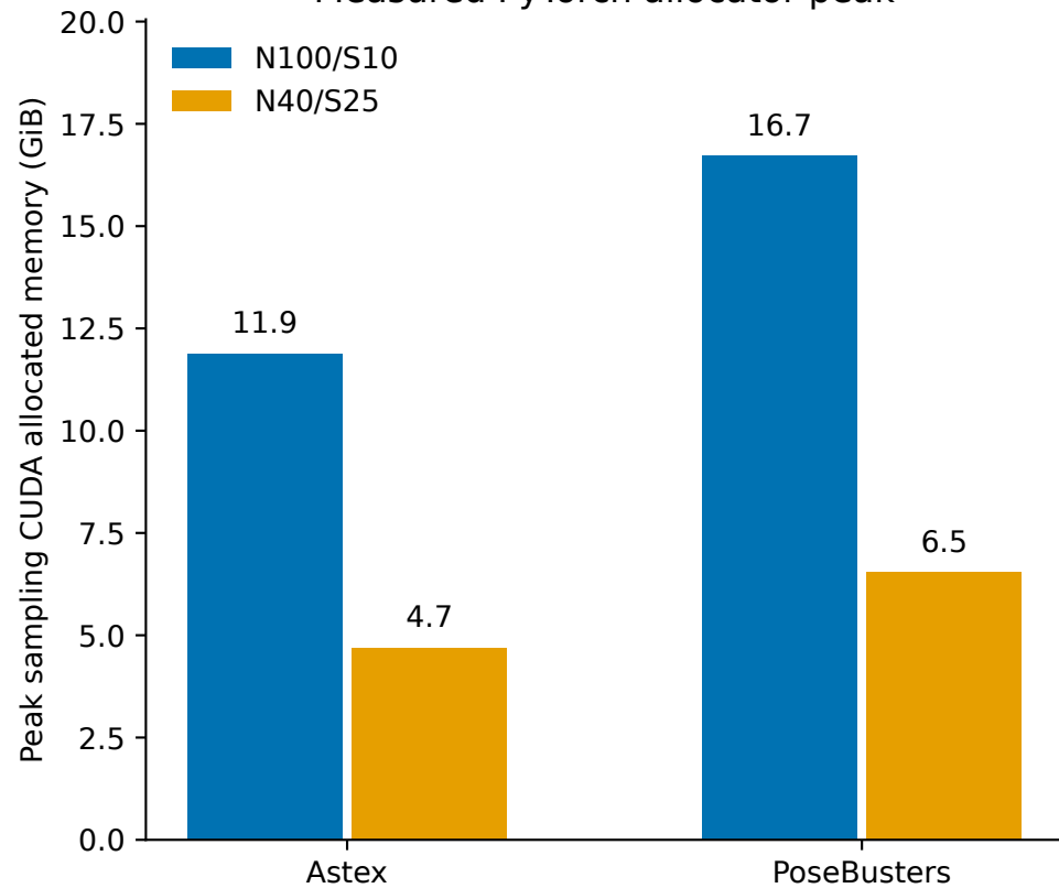
Measured PyTorch allocator peak
