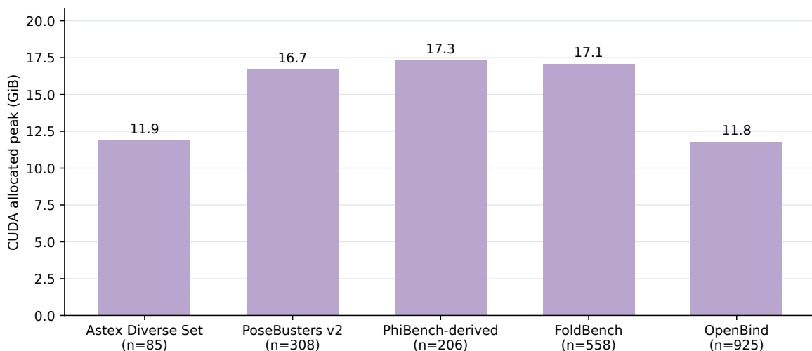
Figure S5: Initial pose-generation process memory. Maximum CUDA allocated-memory peak across shards and three repeats of the initial unguided 100-pose, 10-step evaluation. This is the original generation/evaluation process allocator peak, not reserved memory or a whole-pipeline peak. Astex and PoseBusters used candidate-only generation processes, whereas PhiBench-derived, FoldBench and OpenBind processes included initial confidence scoring. The later correction stages are excluded. Mixed devices and these different process profiles preclude a controlled comparison of sampling-only memory.
