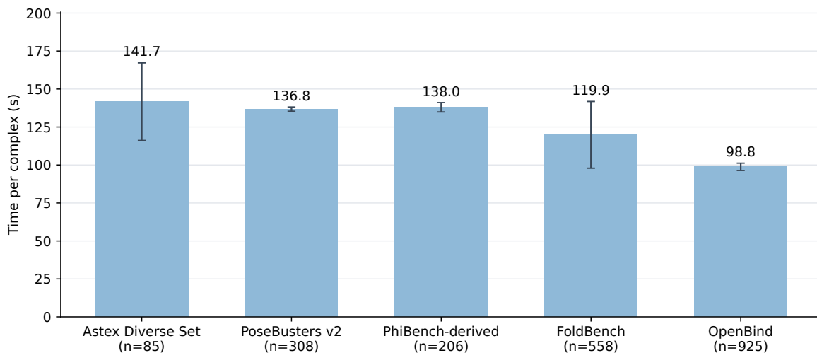
Figure S4: Initial candidate-acquisition pipeline runtime. Mean wall time per complex for the unguided 100-pose, 10-step evaluation. These original executions used the corrected orientation operator before the downstream conformer-template and frame-recovery corrections. Runtime includes setup, generation, the original refinement and confidence scoring, and I/O; it excludes separately executed official PoseBusters evaluation and the later correction stages. Whiskers show sample SD across three fixed-weight inference repeats. Mixed devices and cohort-specific process profiles preclude a controlled speed comparison.
