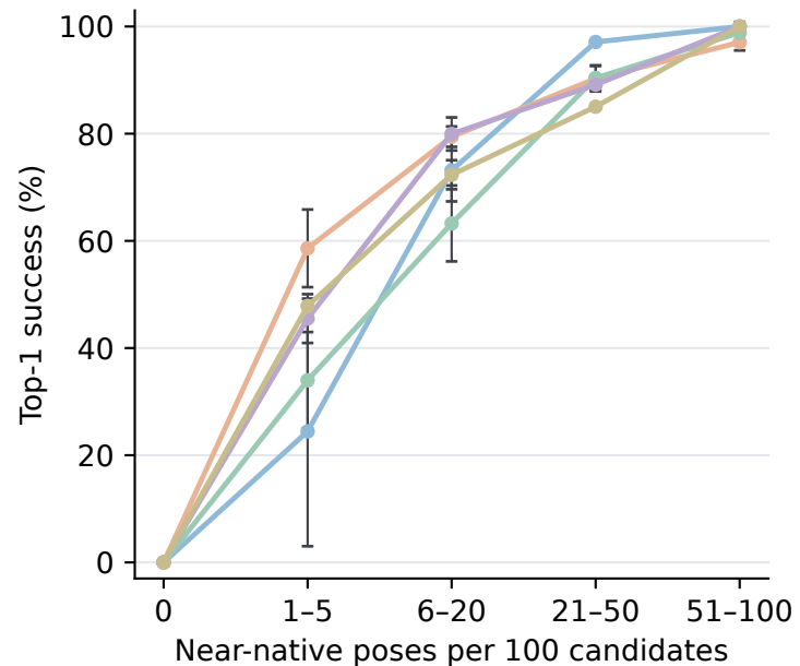
C Near-native candidate density
