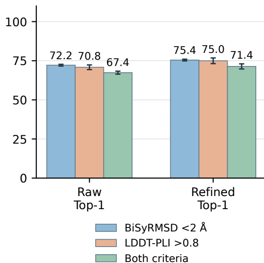
B FoldBench (n=558)
