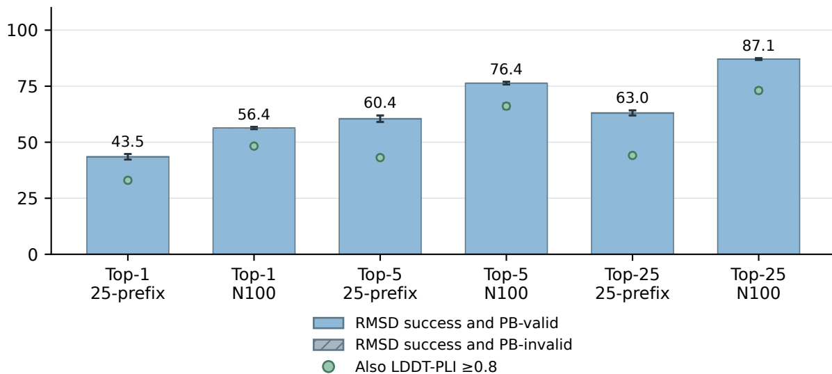
C OpenBind follow-on (n=802)
