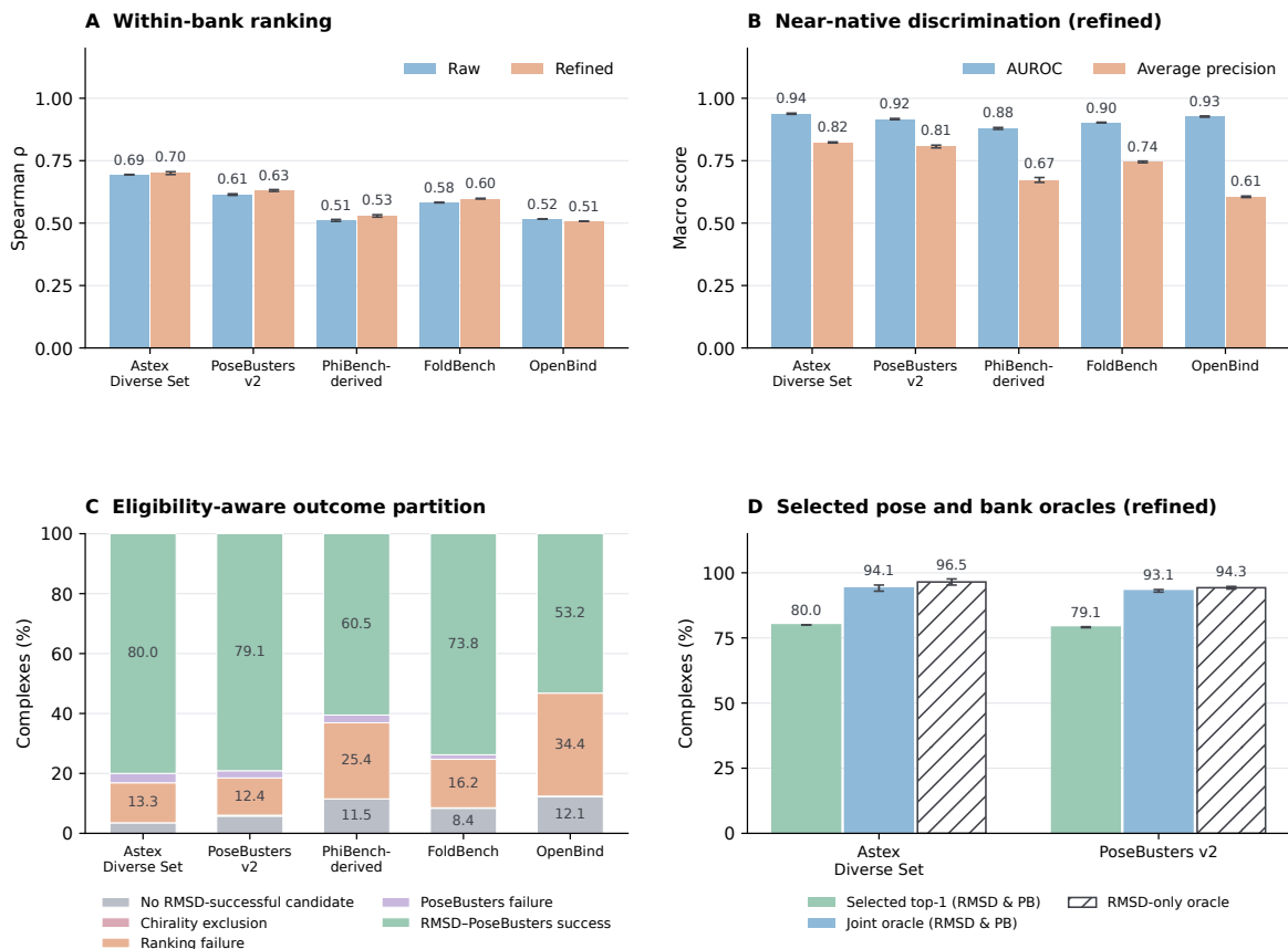
Figure 5: Confidence ranking and selection headroom. (A) Within-complex Spearman correlation between predicted and observed RMSD for raw and refined banks. (B) Refined-bank AUROC and average precision for RMSD < 2 Å labels; banks containing only one class are excluded. (C) Partition of refined primary outcomes: no RMSD-successful candidate in the bank; all such candidates excluded by the chirality screen; an eligible RMSD-successful candidate not selected (ranking failure); the selected RMSD-successful pose fails PoseBusters; or RMSD-PoseBusters success. Candidate success in C is defined by RMSD alone. (D) For Astex and PoseBusters v2, selected-pose RMSD-PoseBusters success compared with the joint oracle (any candidate with RMSD < 2 Å passing all PoseBusters checks) and the RMSD-only oracle, from official checks on every refined candidate. Bars show three-repeat means and sample SD.
