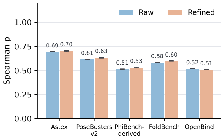
A Within-bank ranking
