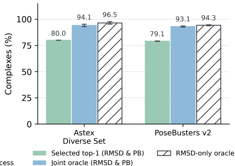
D Selected pose and bank oracles (refined)
