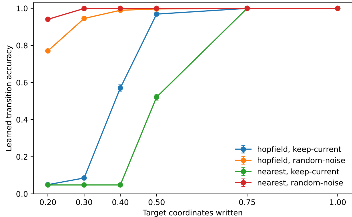
Sparse learned transition proposals
