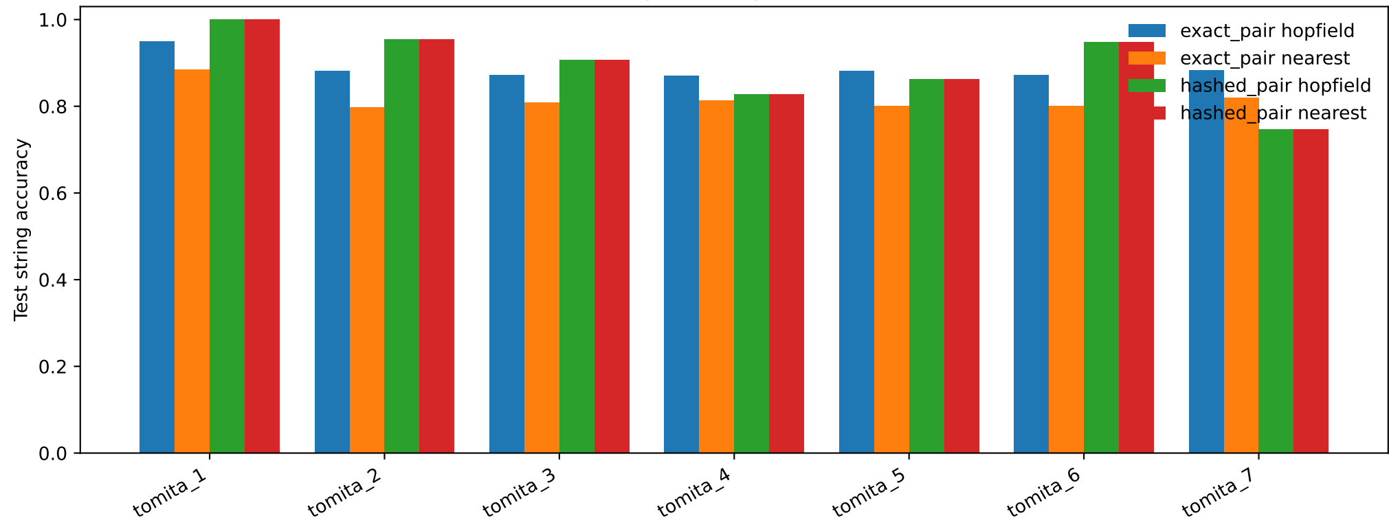
Tomita grammar generalization
