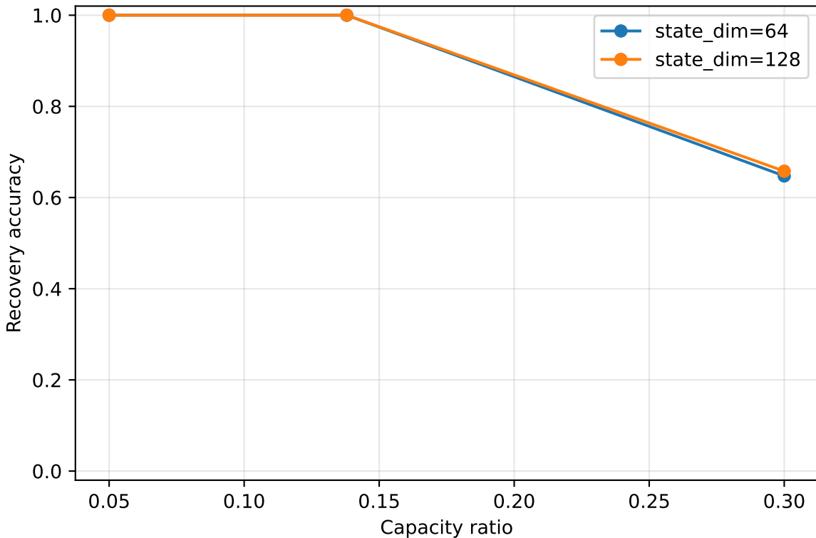
Capacity sweep (hopfield)
