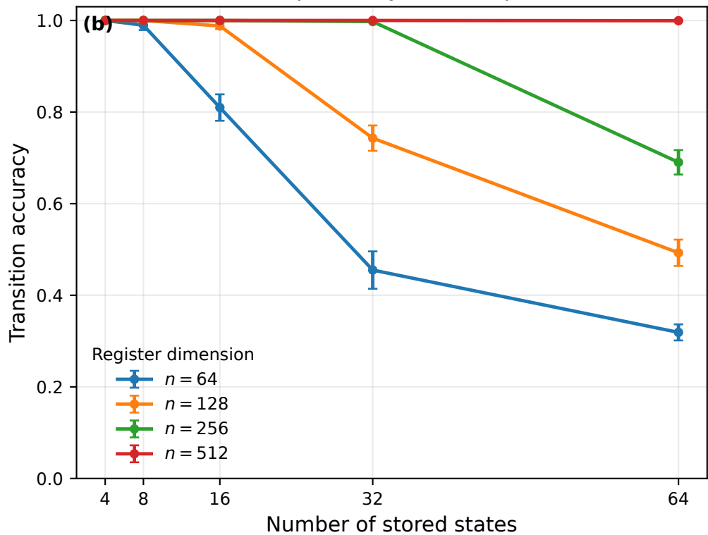
Hopfield-style cleanup
