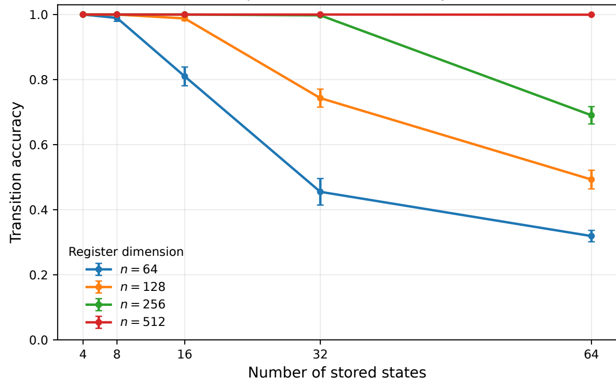
Hopfield transition accuracy
