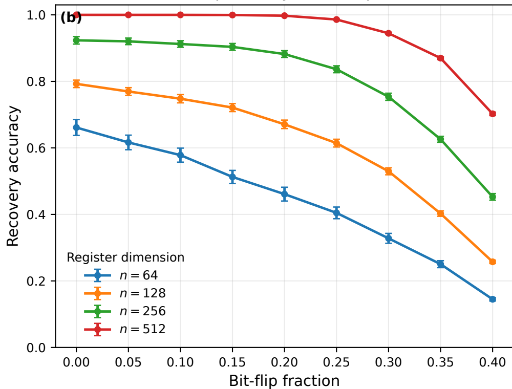
Hopfield-style cleanup
