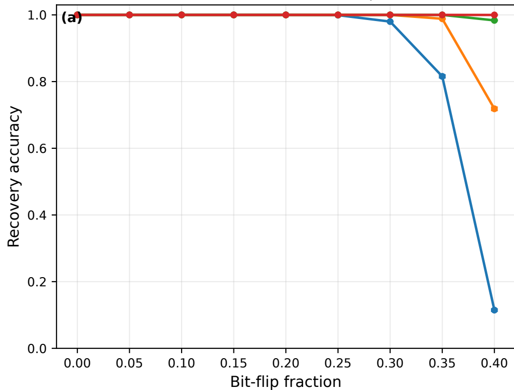
Ideal nearest-attractor cleanup ( m=32 )
