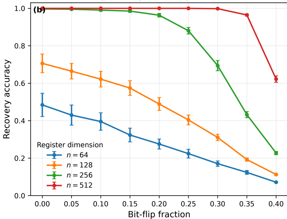
Hopfield-style cleanup ( m=32 )
