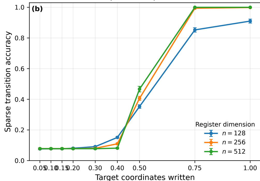
Hopfield, random-noise
