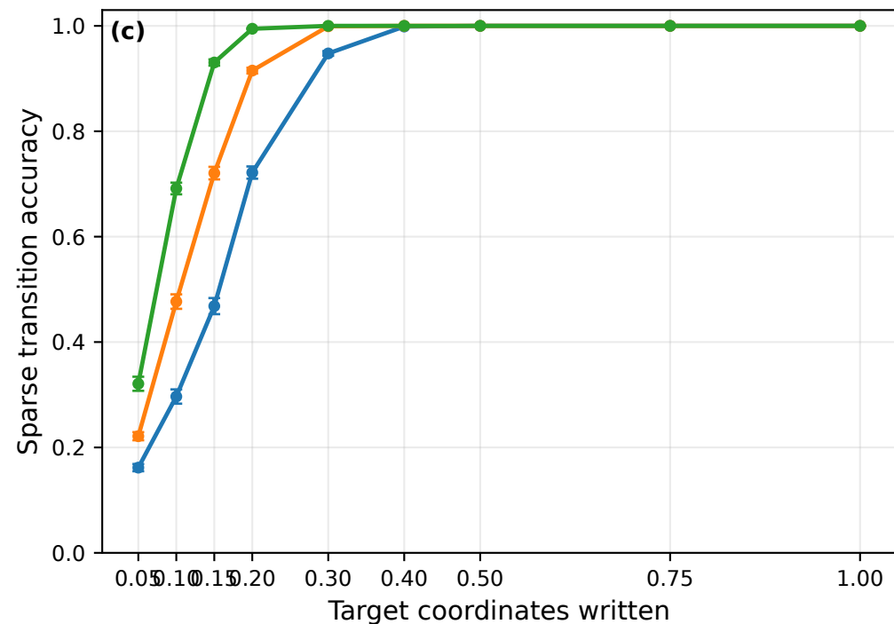
Nearest, random-noise
