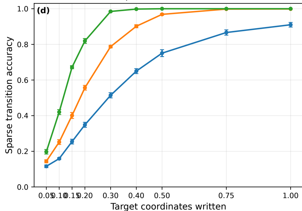
Hopfield, random-noise
