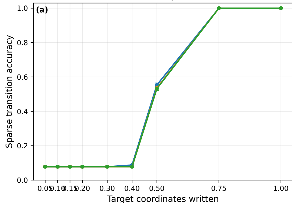
Nearest, random-noise
