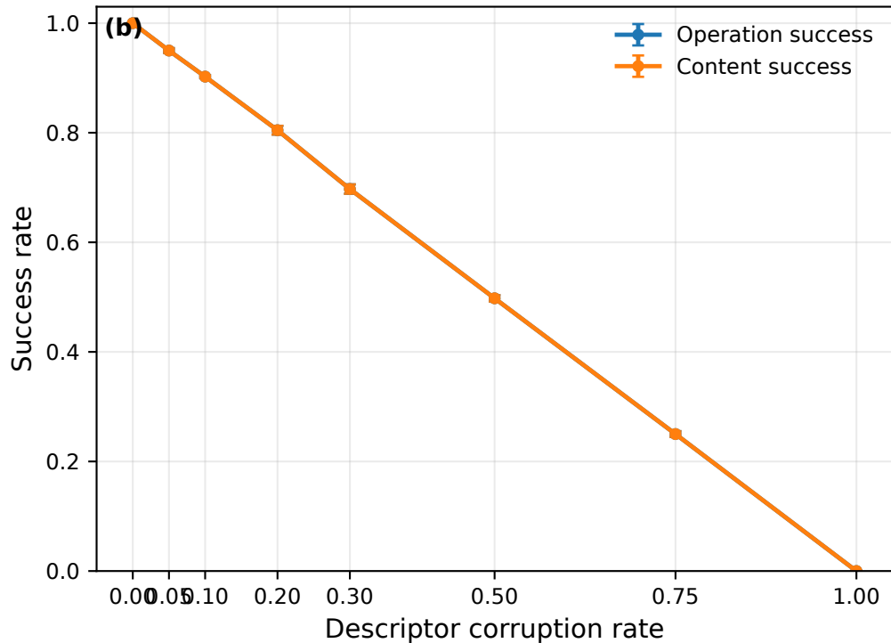
Descriptor corruption affects operation-level success
