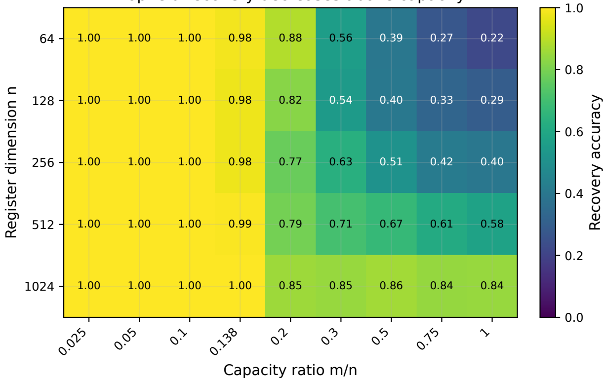
Hopfield recovery decreases above capacity
