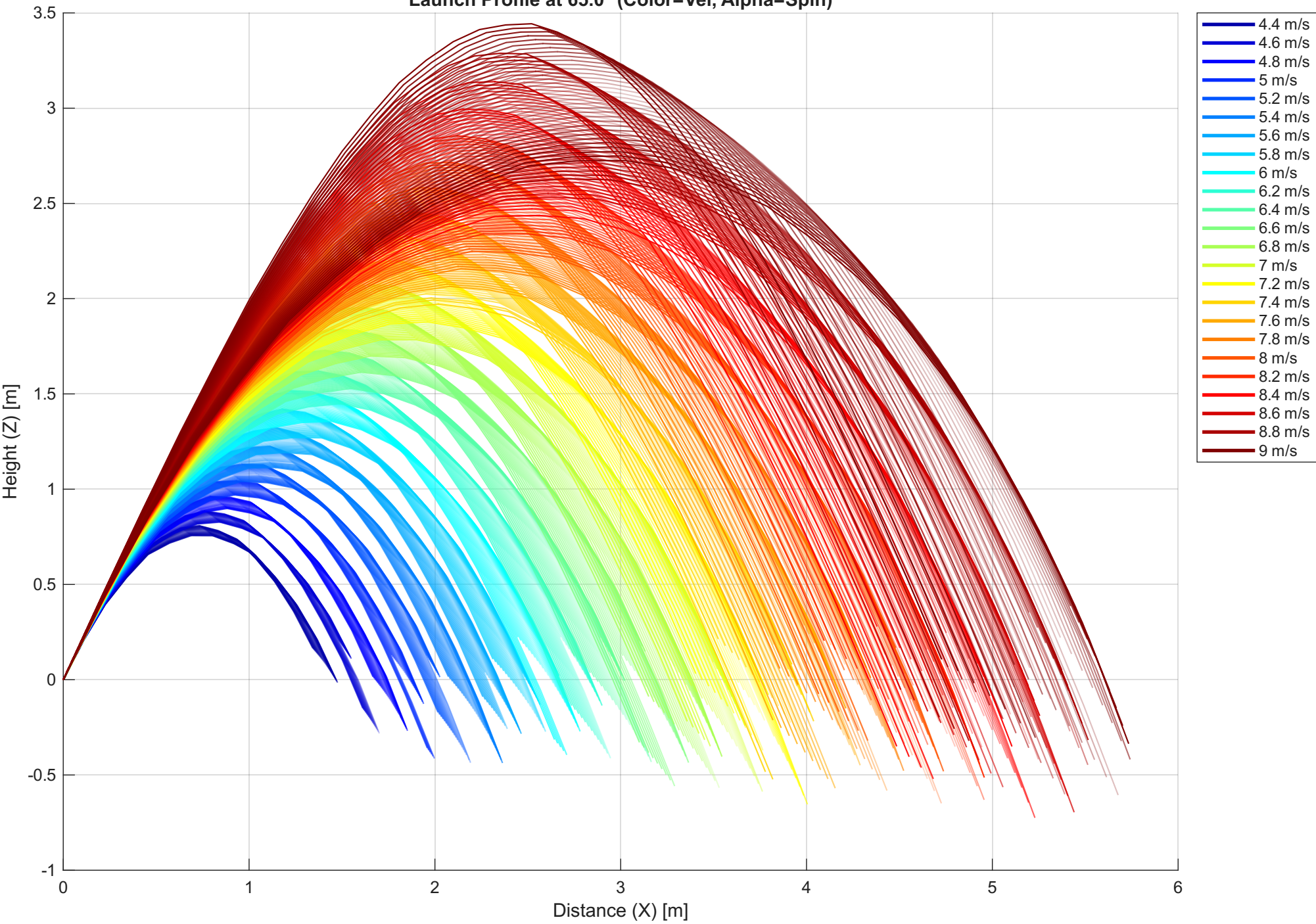
Launch Profile at 65.0° (Color=Vel, Alpha=Spin)
