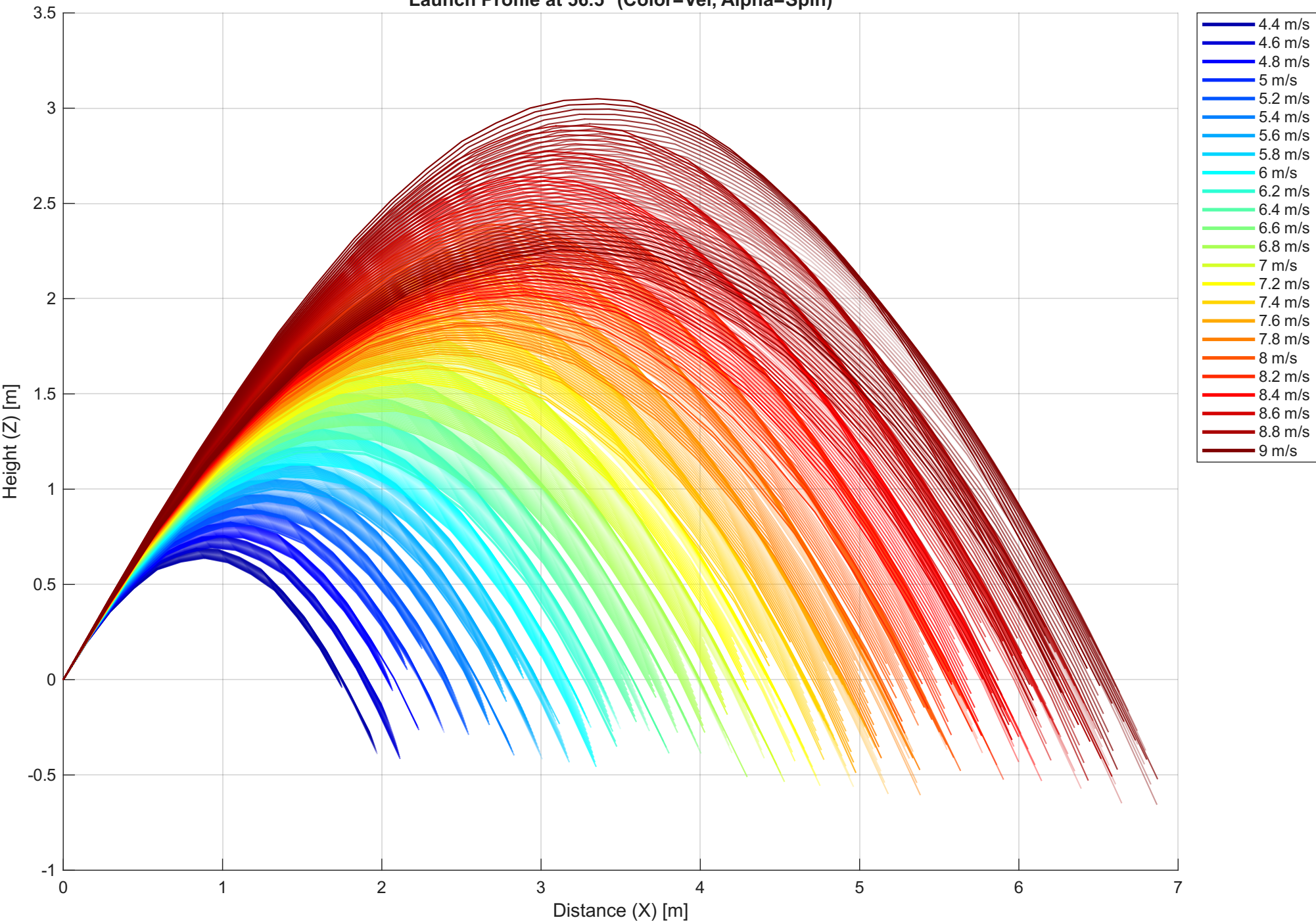
Launch Profile at 56.5° (Color=Vel, Alpha=Spin)
