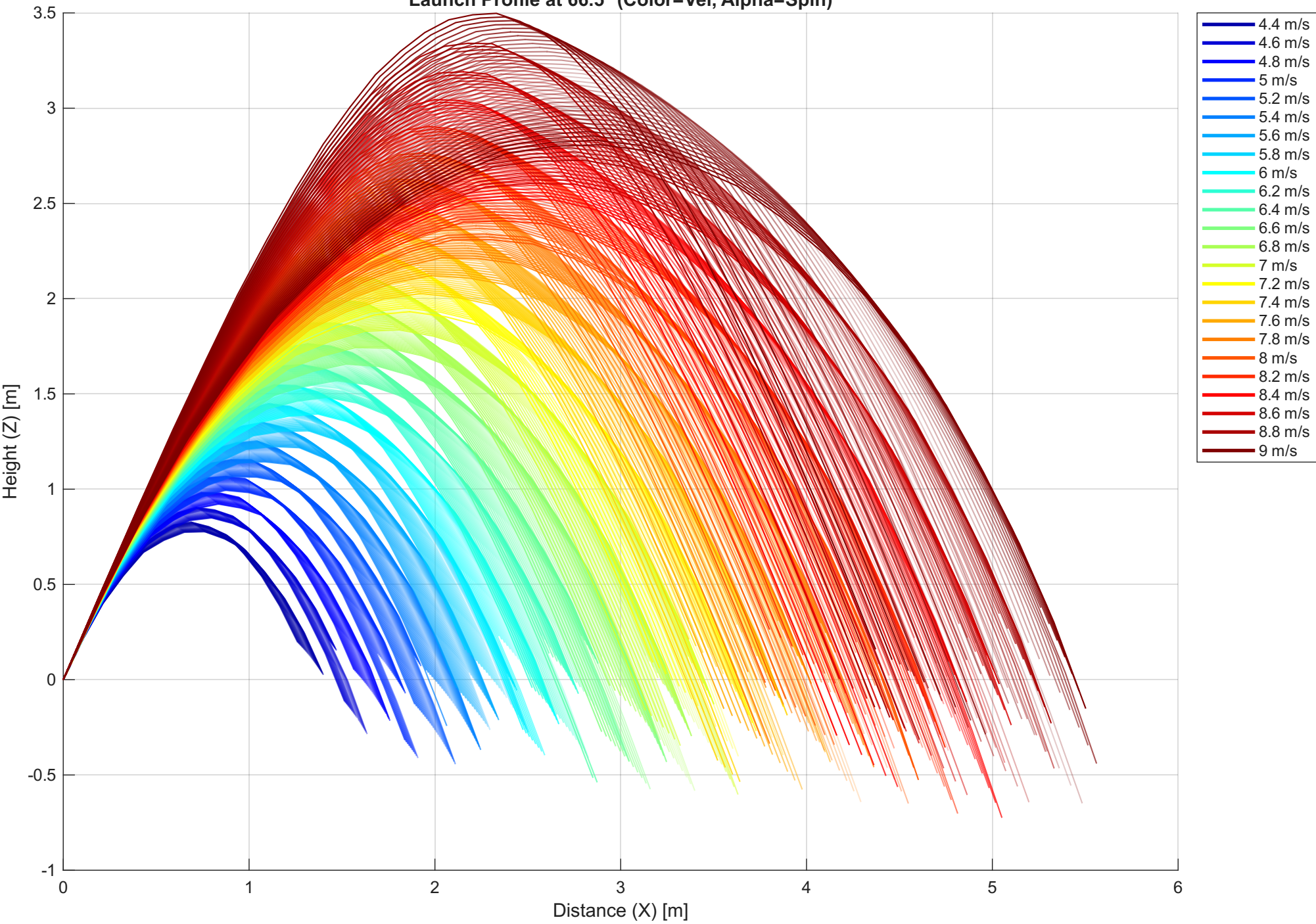
Launch Profile at 66.5° (Color=Vel, Alpha=Spin)
