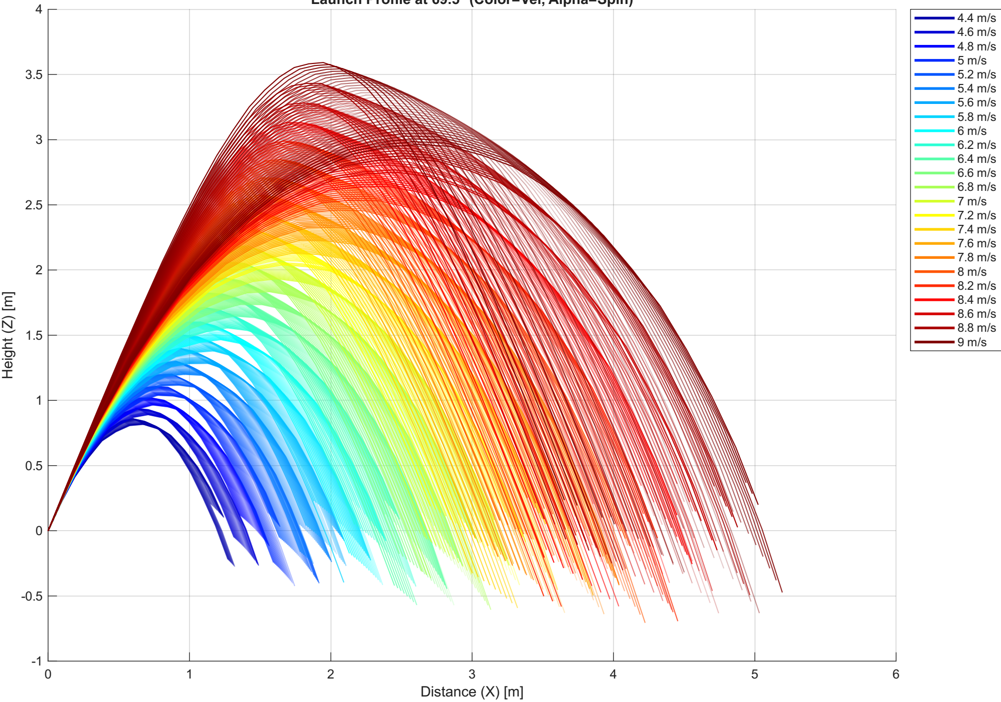
Launch Profile at 69.5° (Color=Vel, Alpha=Spin)
