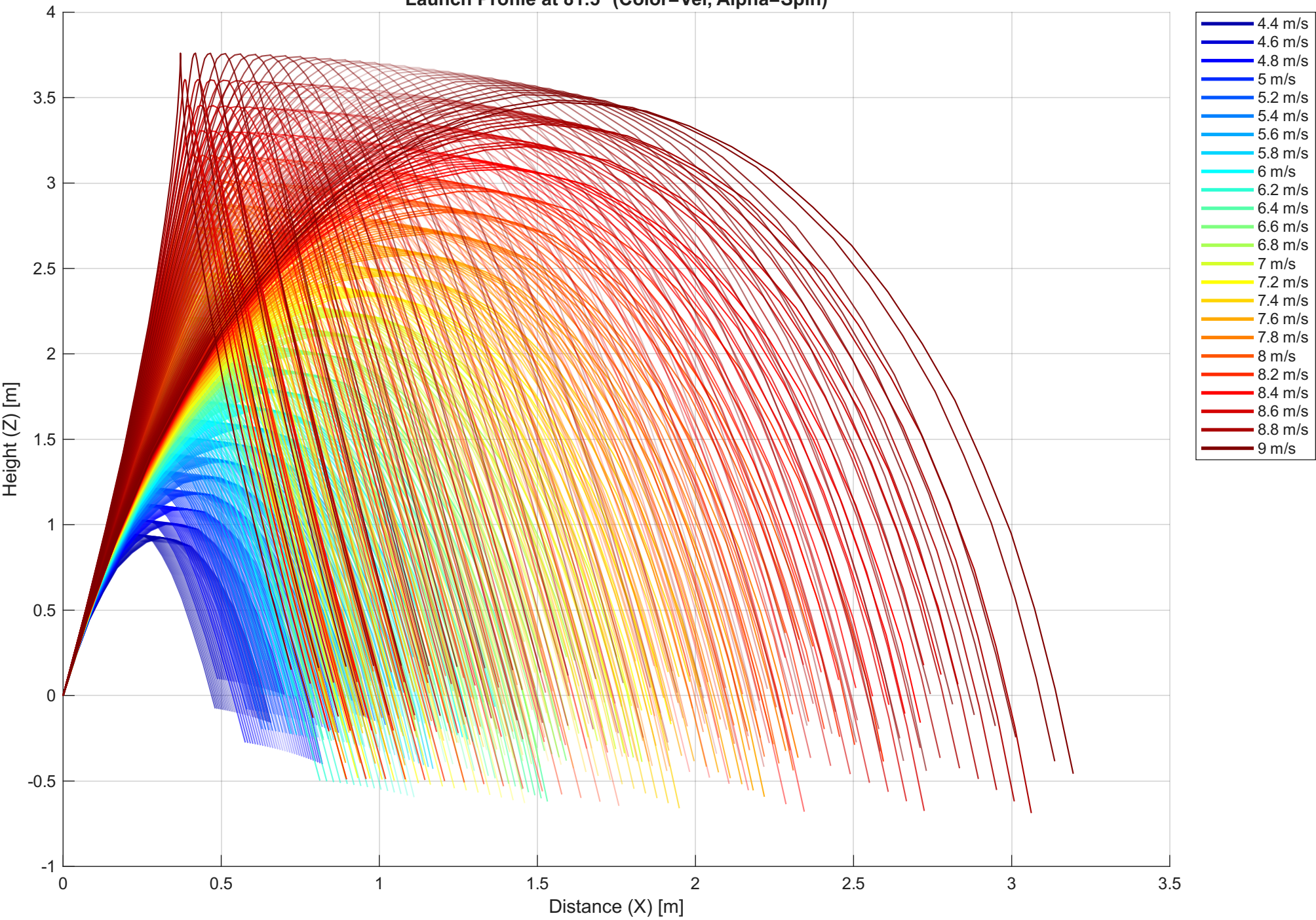
Launch Profile at 81.5° (Color=Vel, Alpha=Spin)
