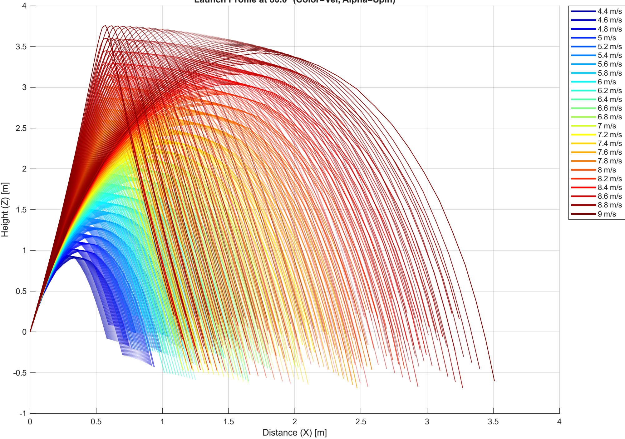
Launch Profile at 80.0° (Color=Vel, Alpha=Spin)
