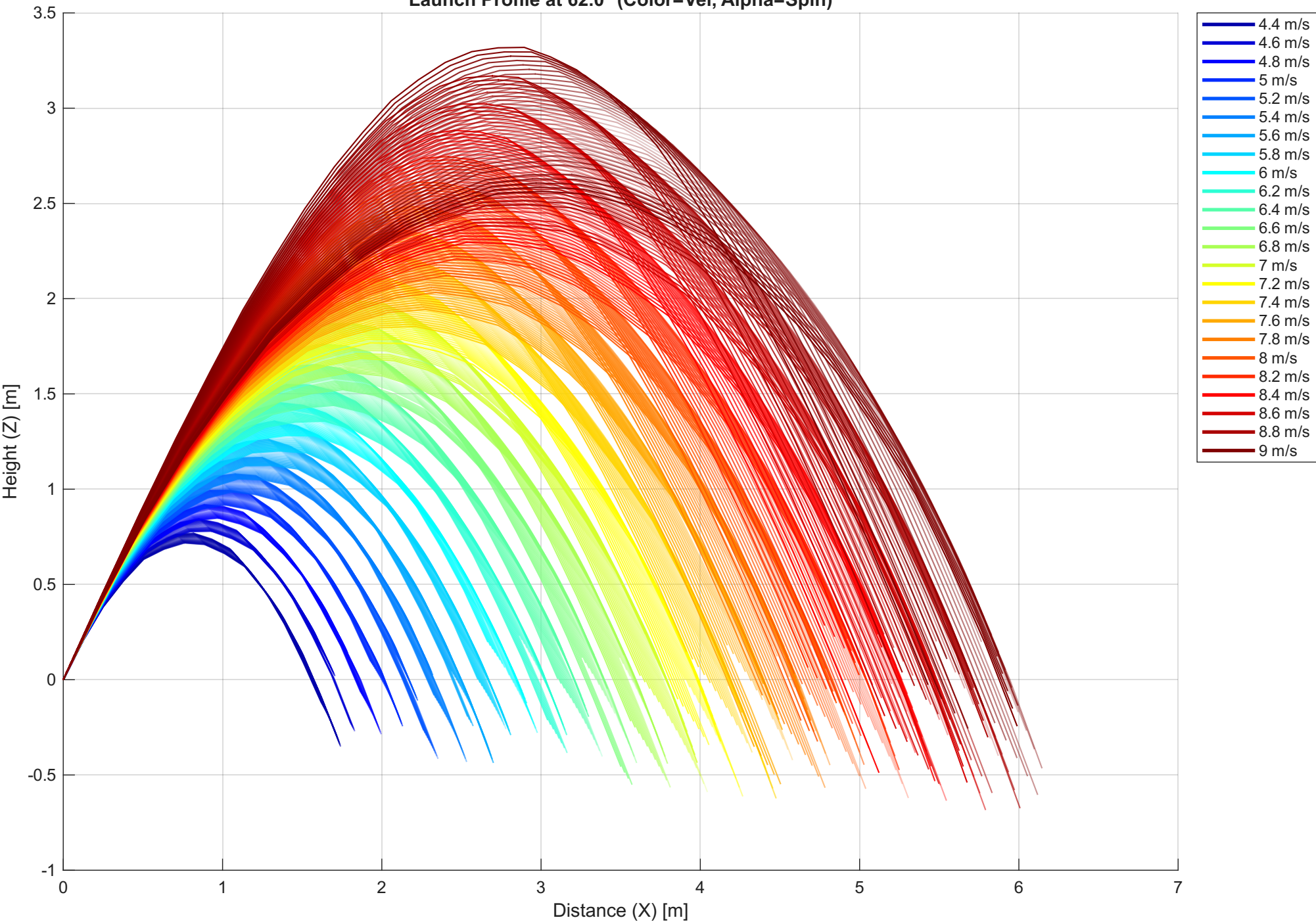
Launch Profile at 62.0° (Color=Vel, Alpha=Spin)
