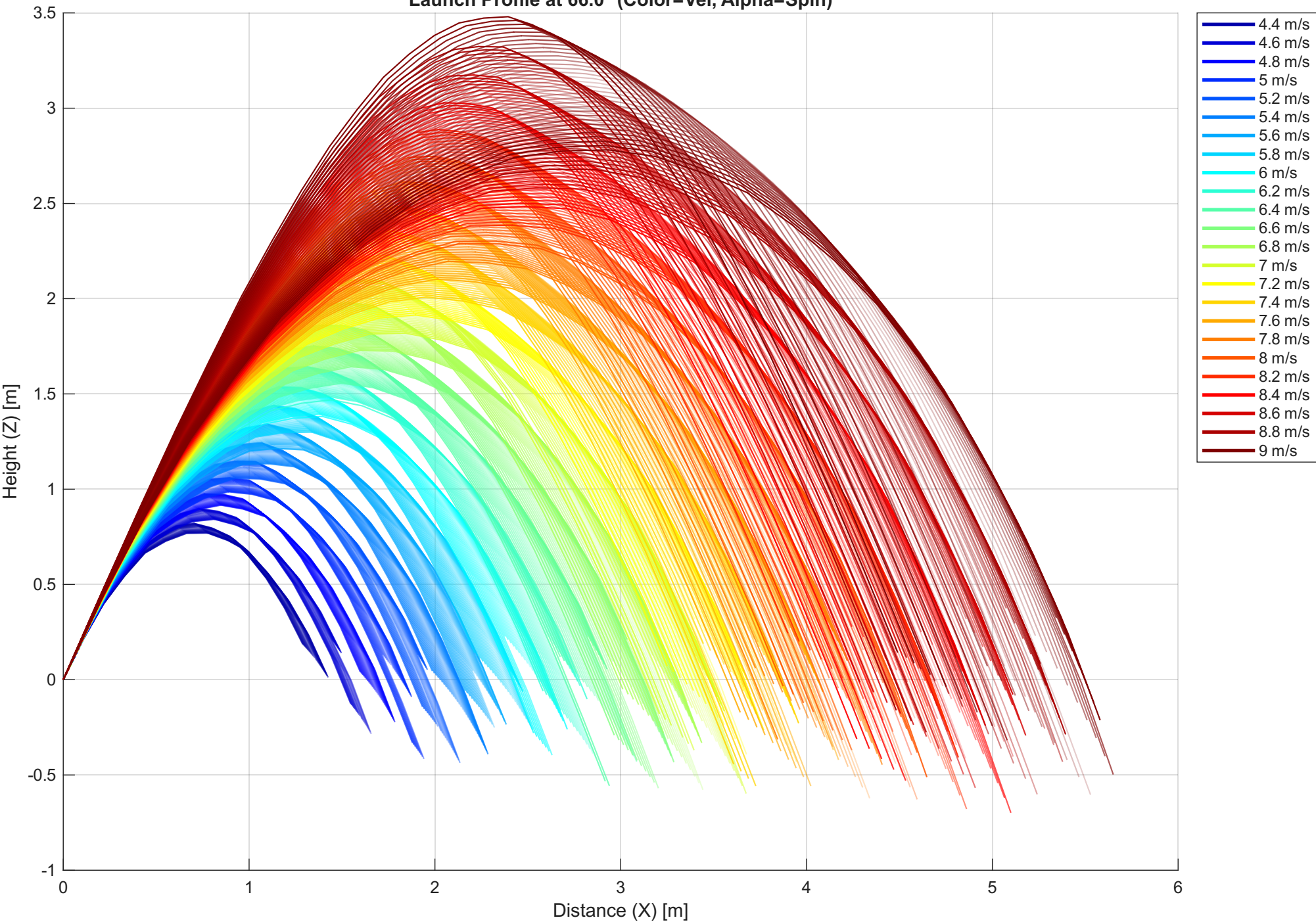
Launch Profile at 66.0° (Color=Vel, Alpha=Spin)
