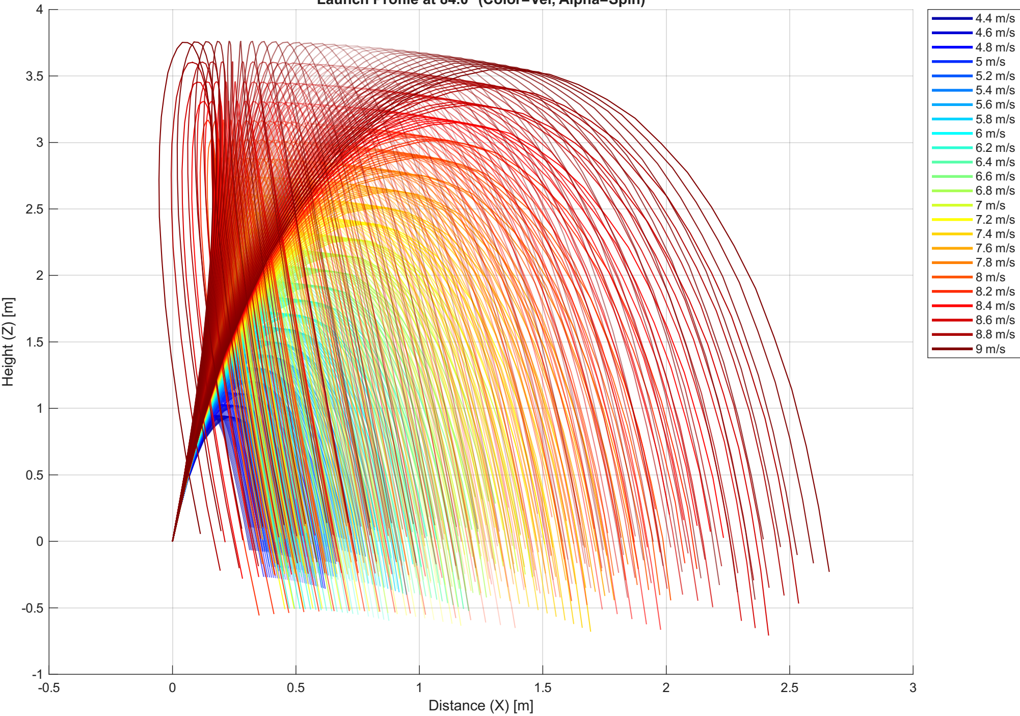
Launch Profile at 84.0° (Color=Vel, Alpha=Spin)
