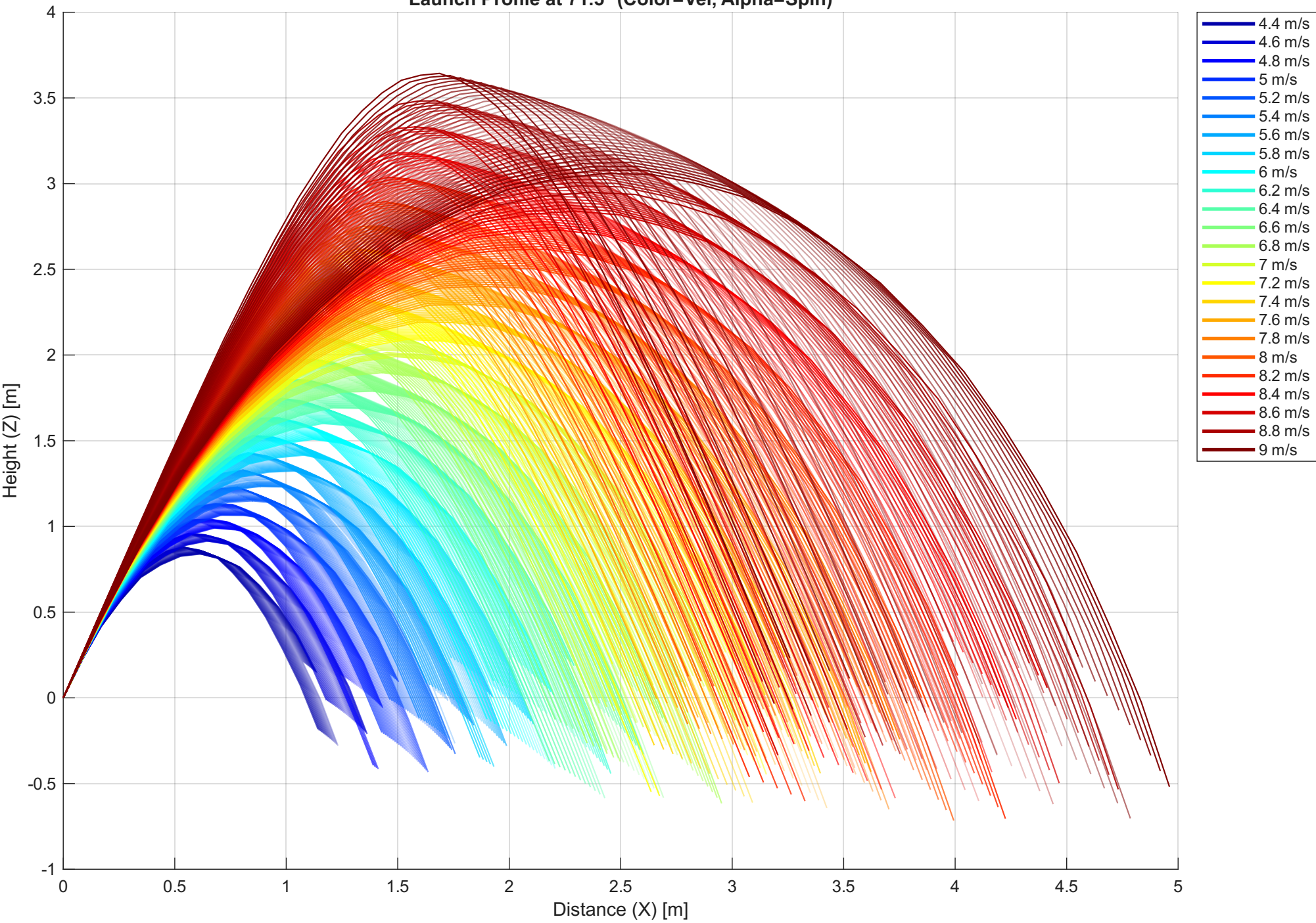
Launch Profile at 71.5° (Color=Vel, Alpha=Spin)
