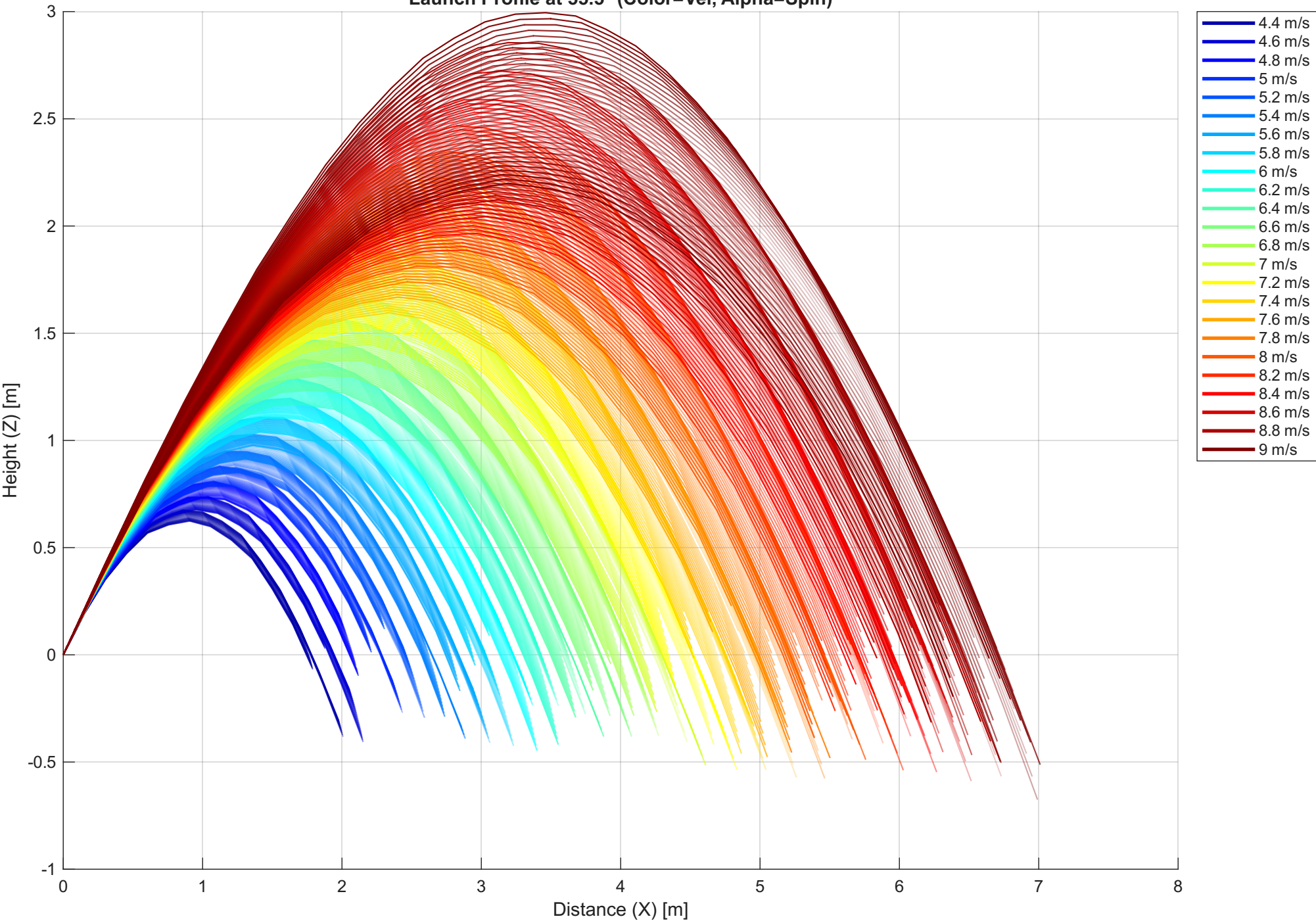
Launch Profile at 55.5° (Color=Vel, Alpha=Spin)
