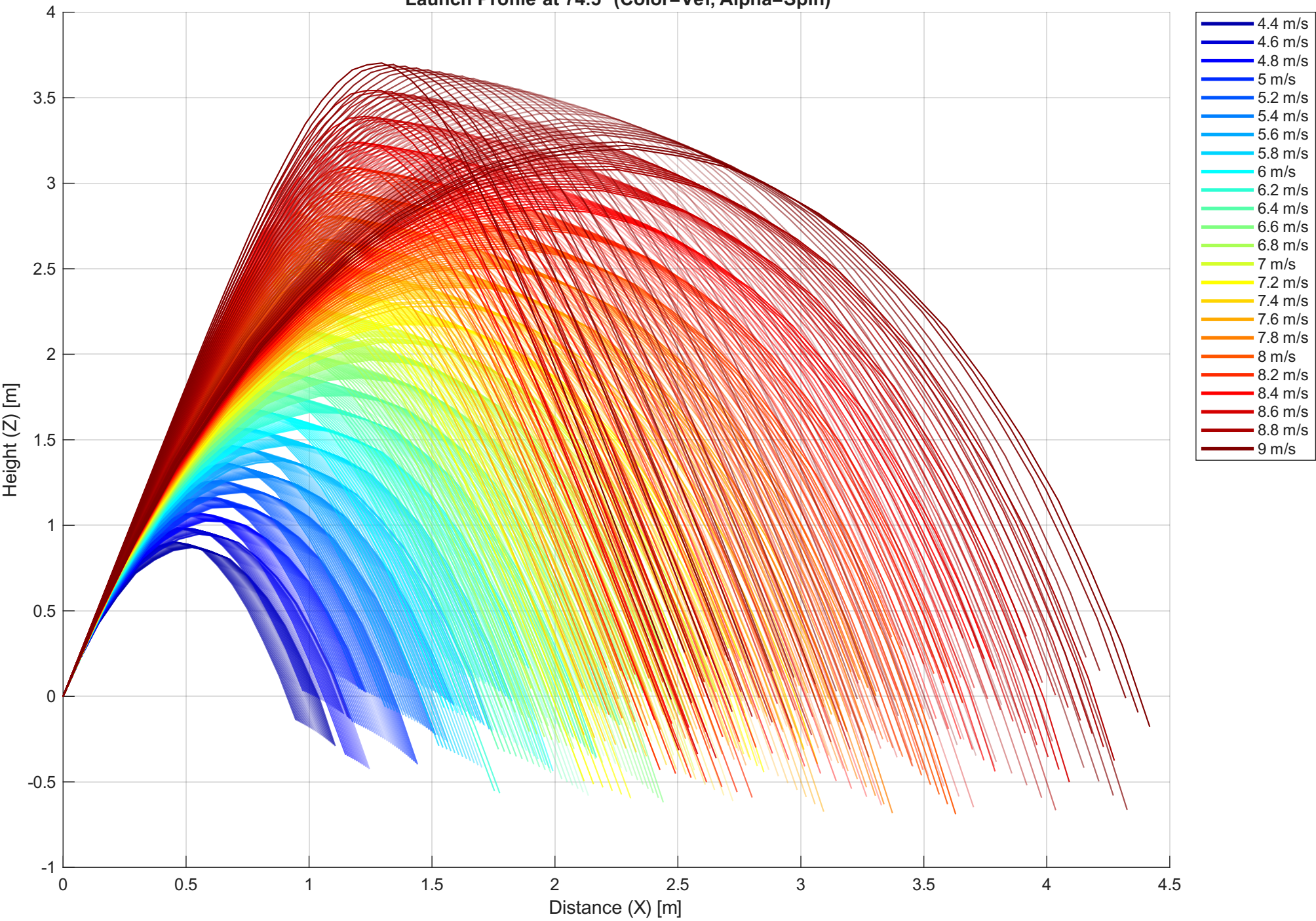
Launch Profile at 74.5° (Color=Vel, Alpha=Spin)
