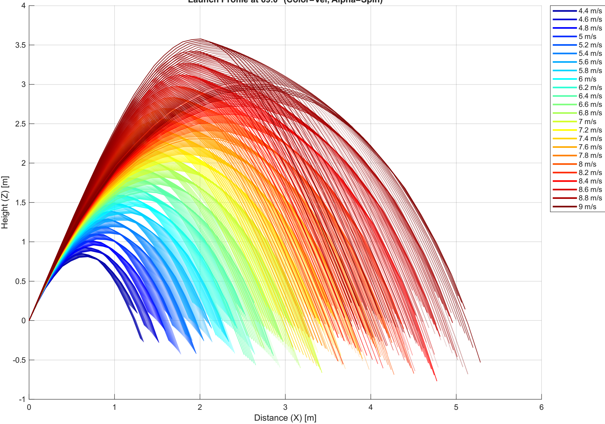
Launch Profile at 69.0° (Color=Vel, Alpha=Spin)
