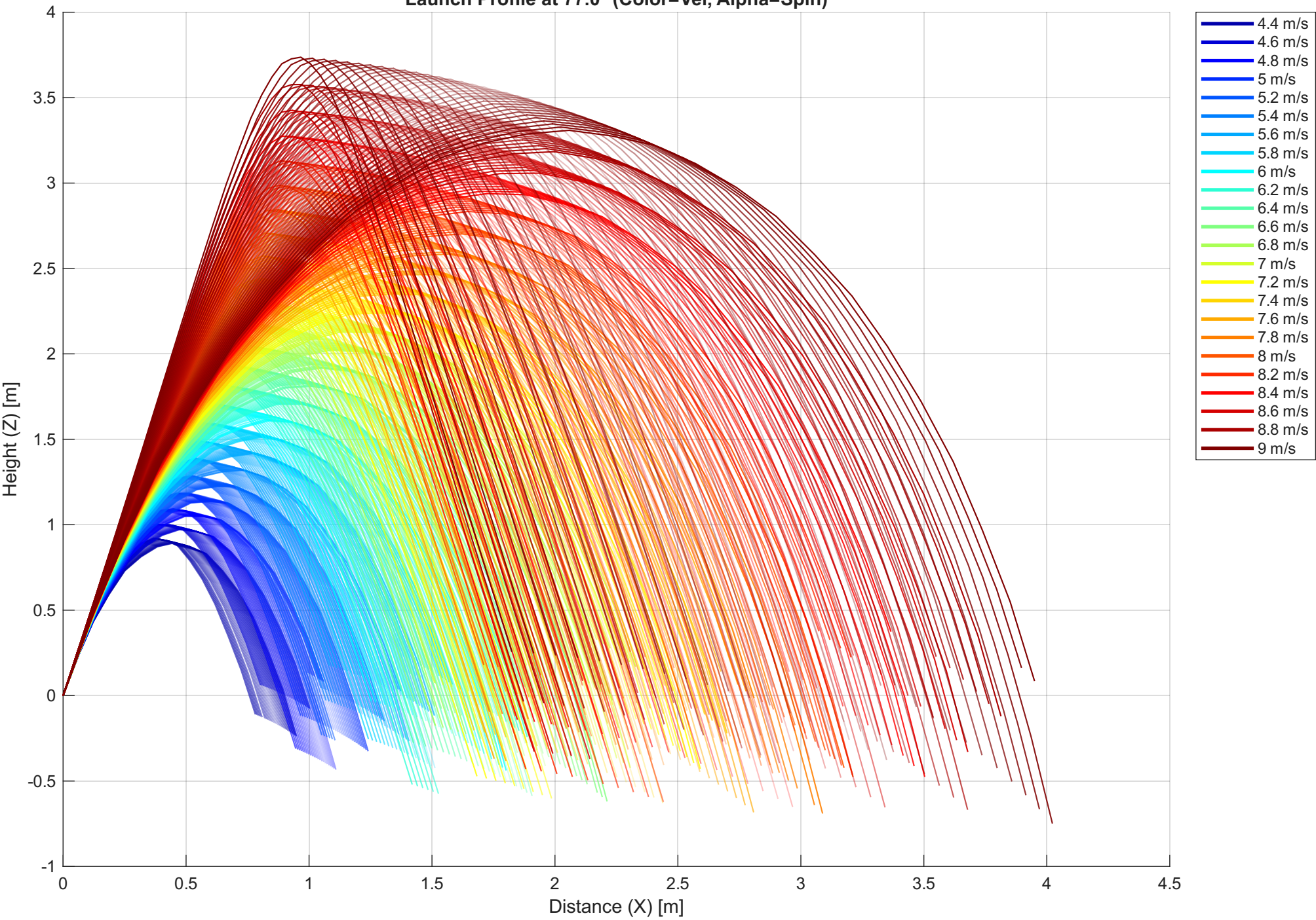
Launch Profile at 77.0° (Color=Vel, Alpha=Spin)
