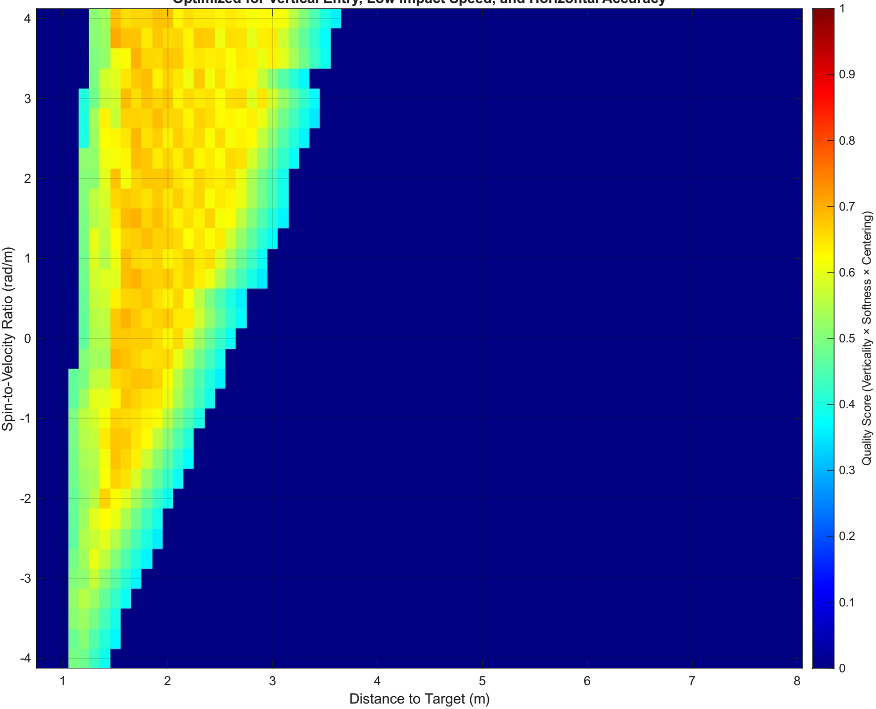
Best-Shot Quality Map | Launch Angle: 80.5° Optimized for Vertical Entry, Low Impact Speed, and Horizontal Accuracy
