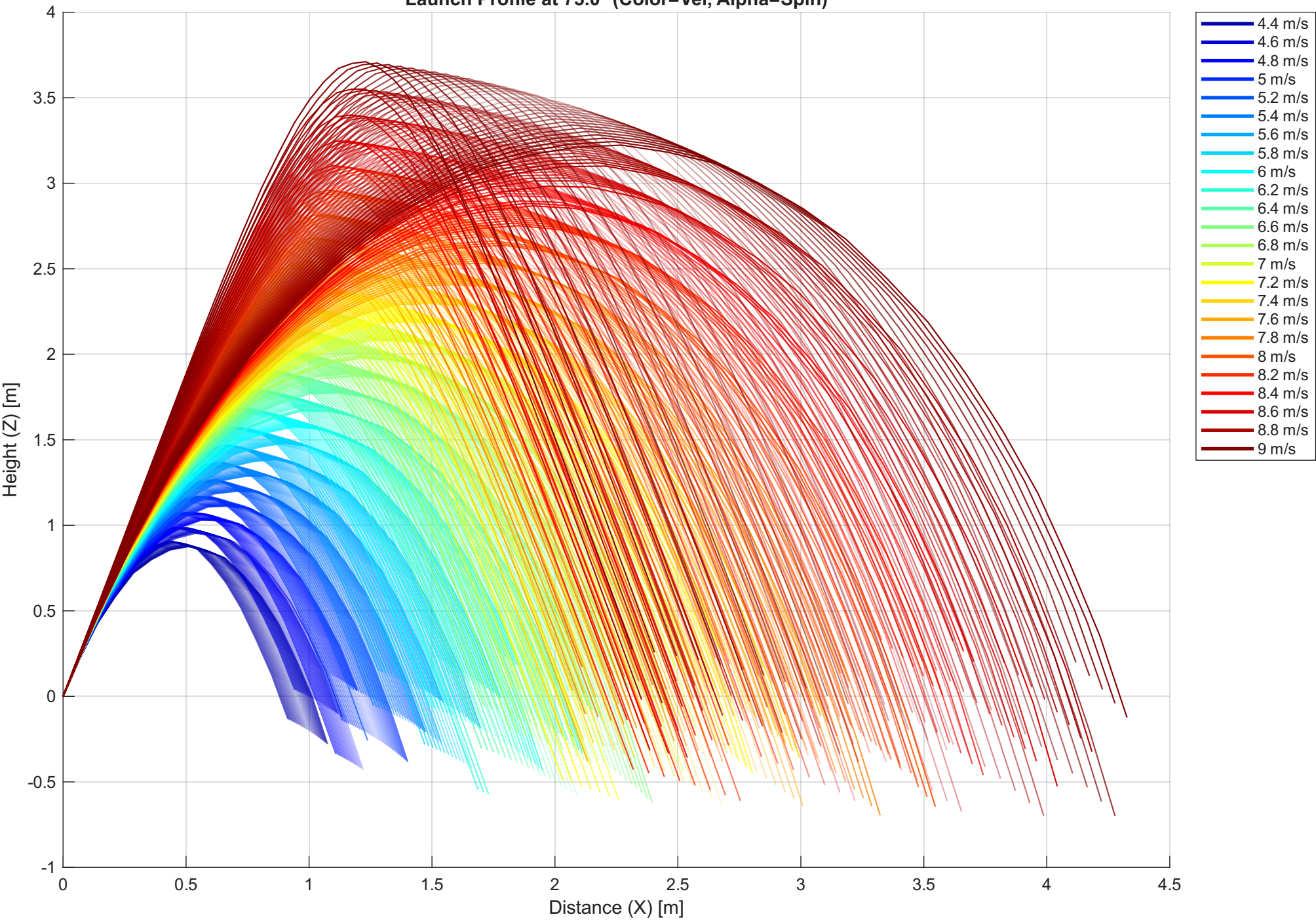
Launch Profile at 75.0° (Color=Vel, Alpha=Spin)
