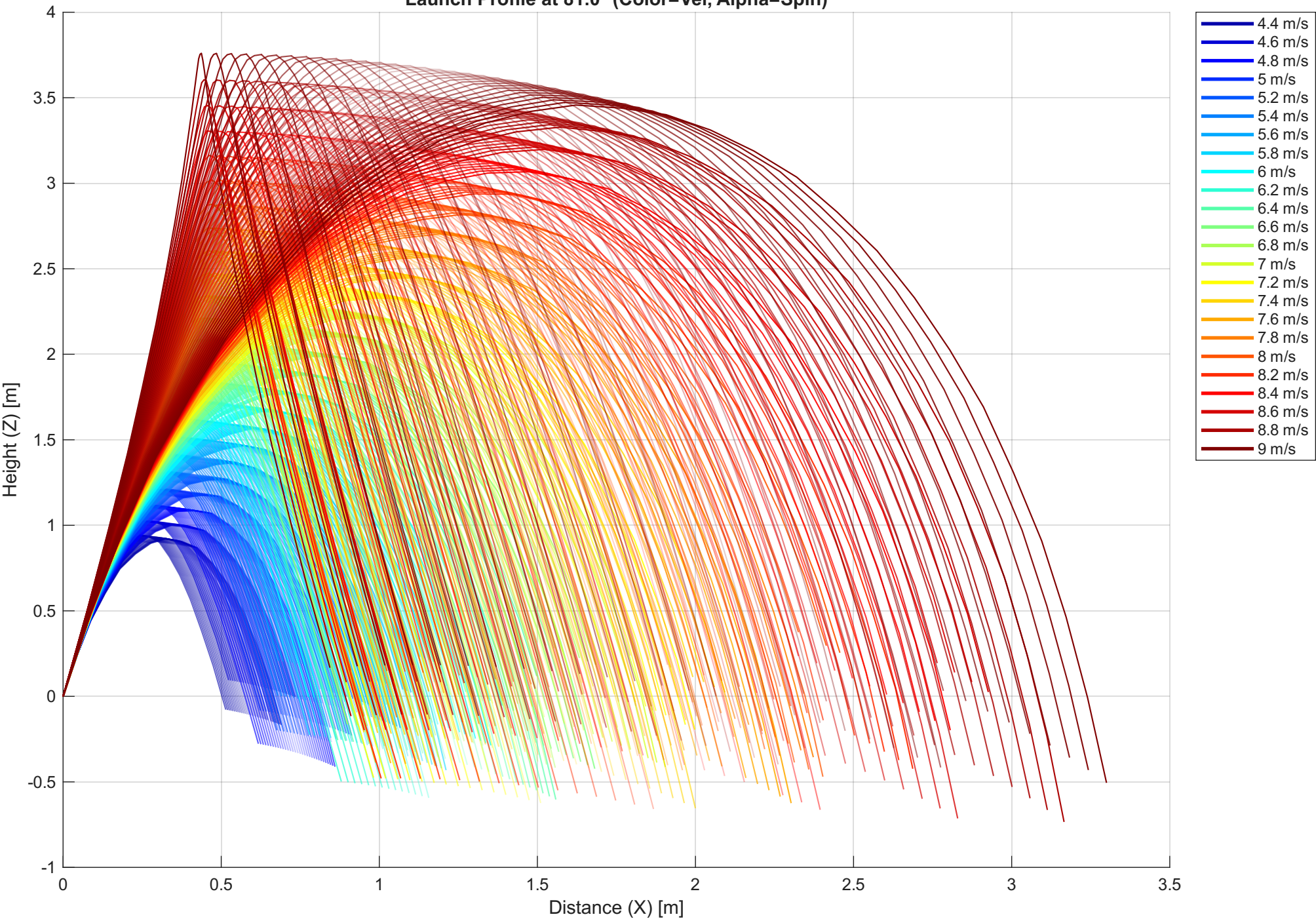
Launch Profile at 81.0° (Color=Vel, Alpha=Spin)
