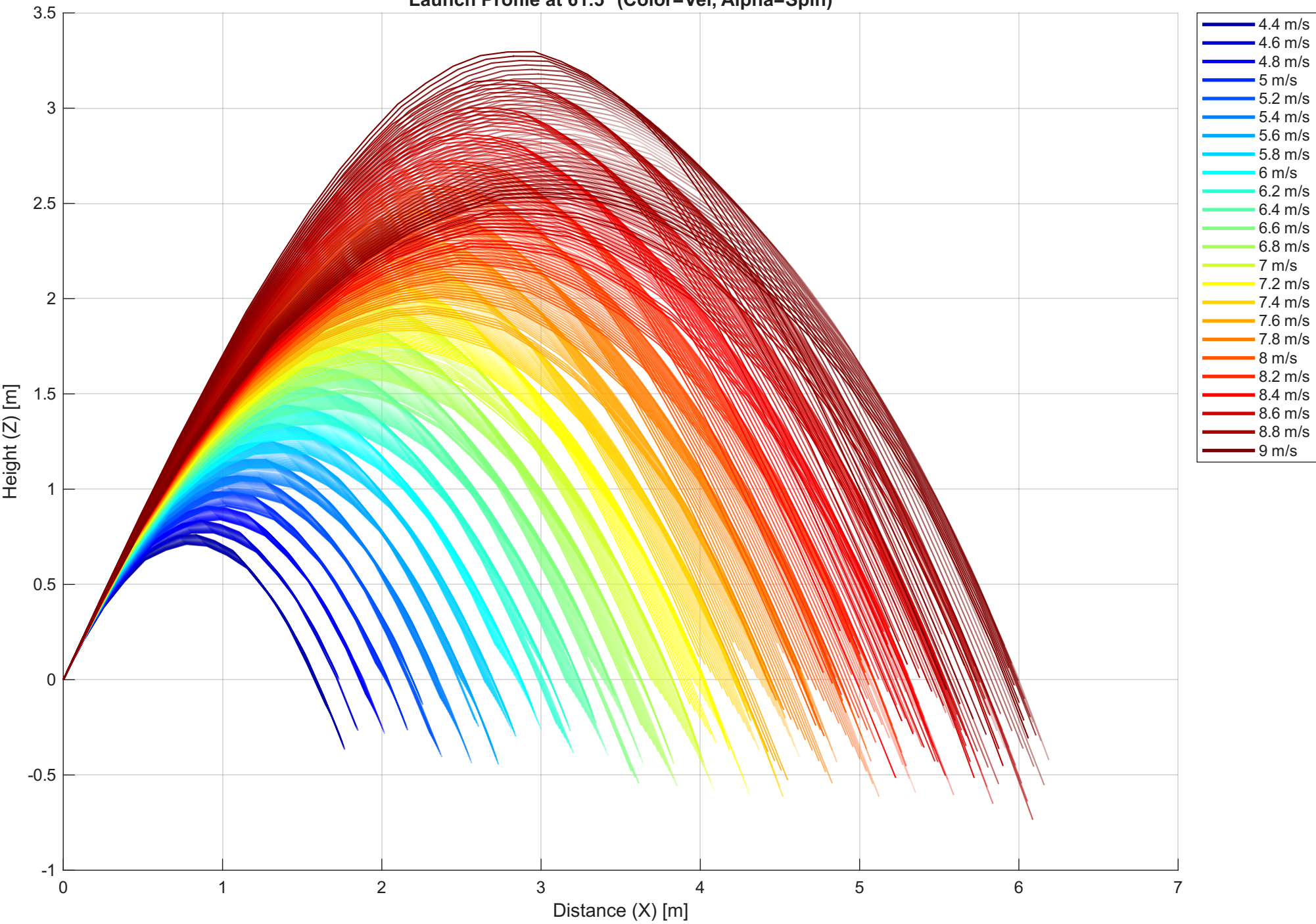
Launch Profile at 61.5° (Color=Vel, Alpha=Spin)
