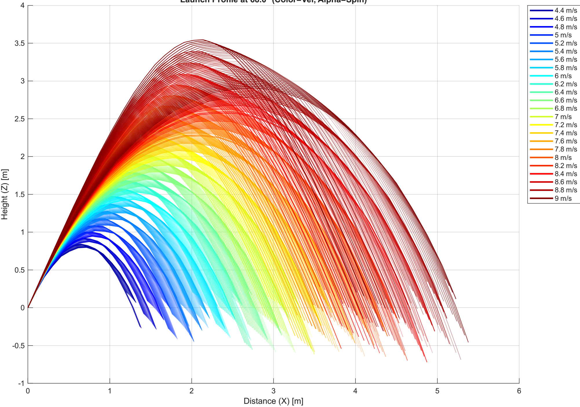
Launch Profile at 68.0° (Color=Vel, Alpha=Spin)
