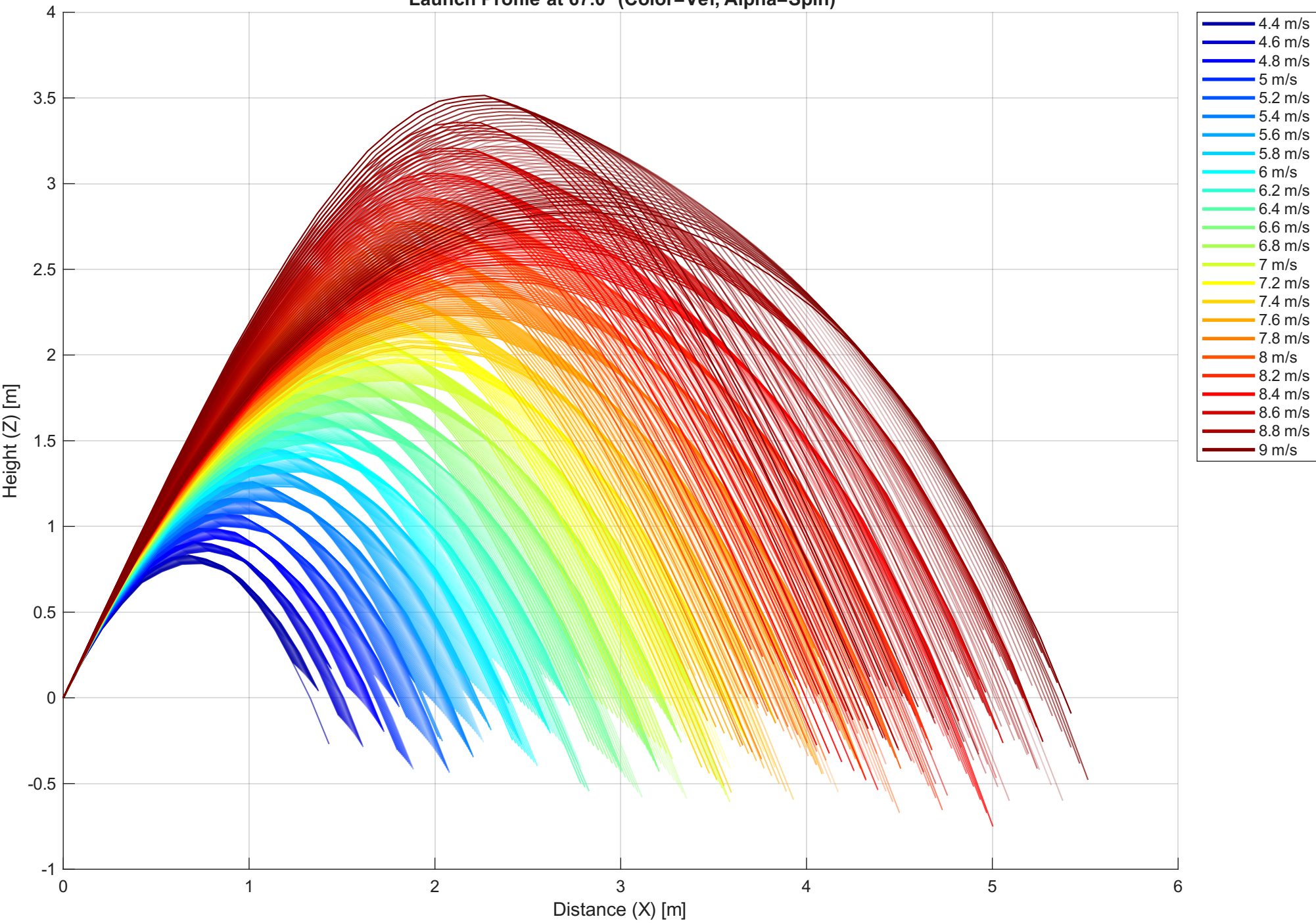
Launch Profile at 67.0° (Color=Vel, Alpha=Spin)
