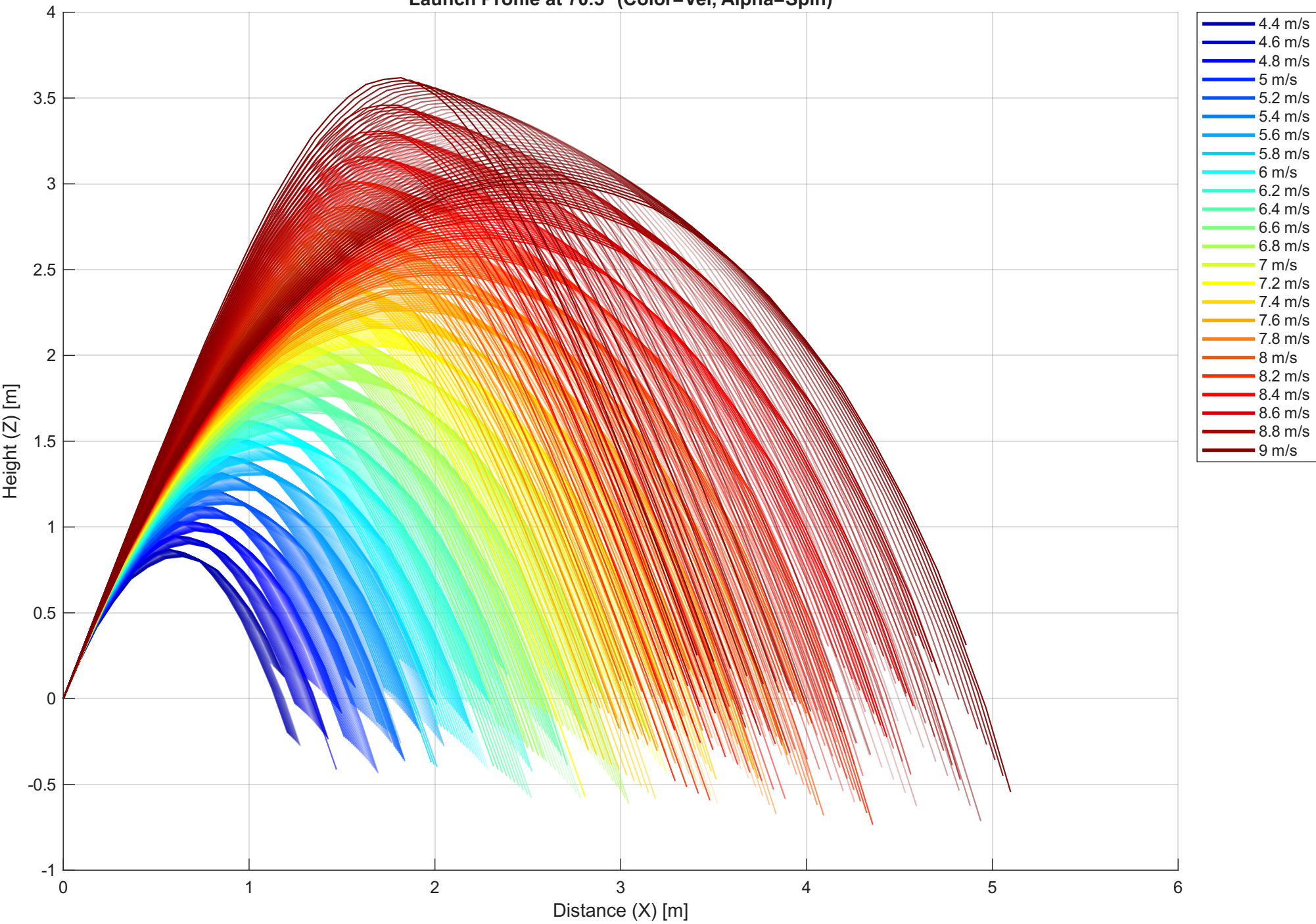
Launch Profile at 70.5° (Color=Vel, Alpha=Spin)
