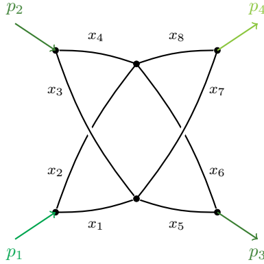
Figure 1: The three-loop Crown with the Schwinger-parameter assignment used in Eq. (38). The external-arrow colours are visual label guides only.
