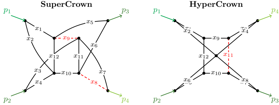
Figure 2: Higher-loop Crown descendants: the five-loop SuperCrown (left) and the four-loop HyperCrown (right). Red dashed edges are set to zero on the contraction strata used in the HR analysis: x_8 = x_9 = 0 for the SuperCrown and x_{11} = 0 for the HyperCrown.
