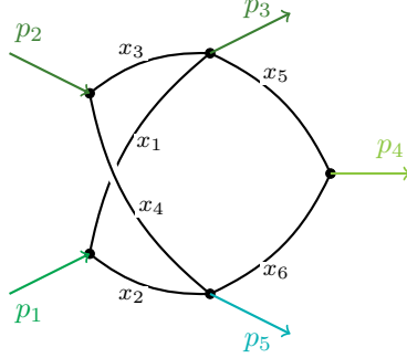
Figure 3: The two-loop five-point seed graph, redrawn in the style of Ref. [5], with the Schwinger parameters used in Eqs. (50)–(54).
