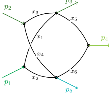
Figure 3: The two-loop five-point seed graph, redrawn in the style of Ref. [5], with the Schwinger parameters used in Eqs. (66)–(70).
