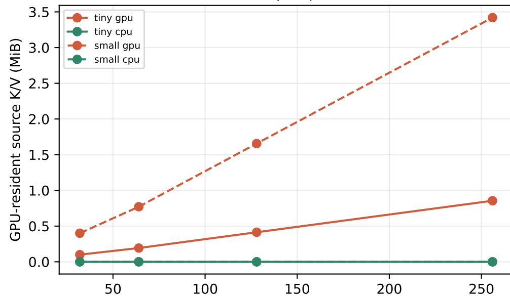
hotpotqa
