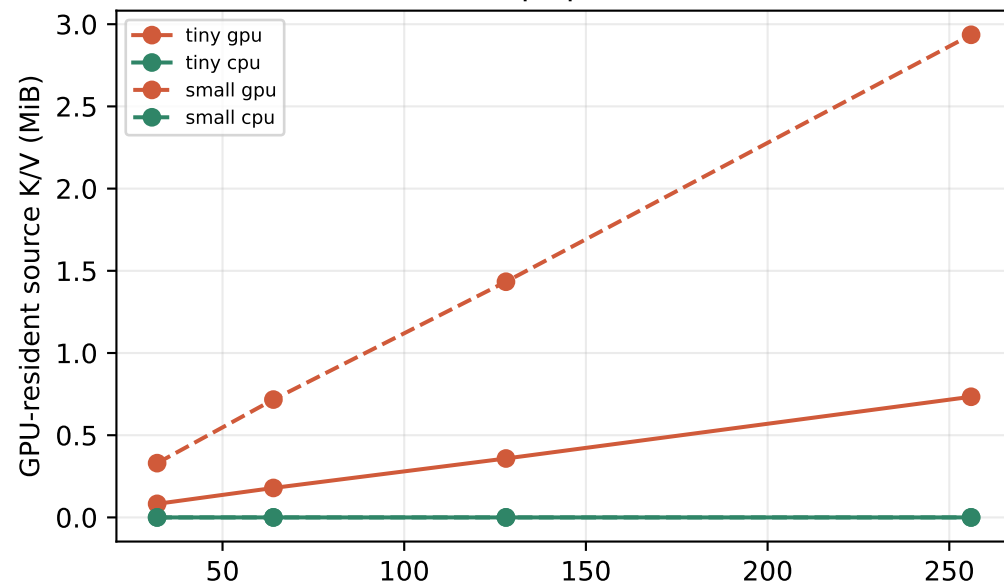
qasper
