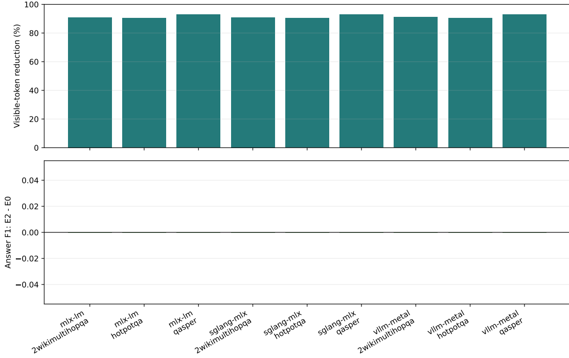
Figure 34: Expanded frozen-selection quality and visible-token accounting. Every engine preserves every paired output; confidence reflects finite sample size.
