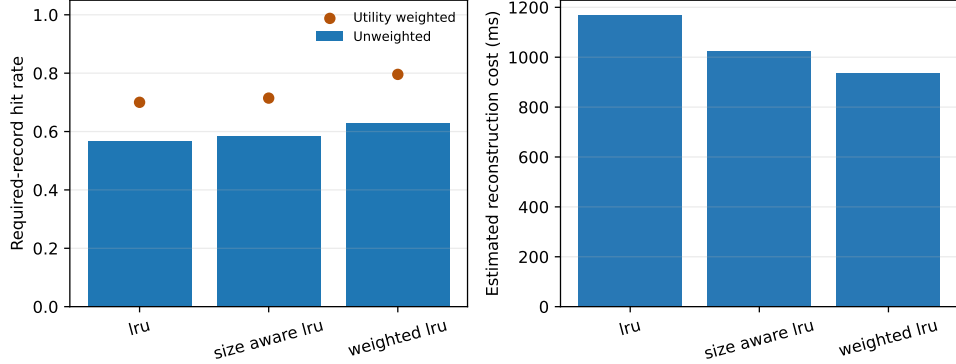
Figure 21: Equal-quota retention on a mixed task, document, and tool-result trace. Weighted policy protects active task state and shared documents while allowing reconstructable transient records to churn.
