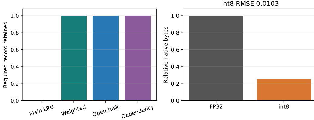
Figure 22: Engine-neutral retention controls and generic symmetric-int8 byte transport. The int8 result is a codec diagnostic; model-specific quality and active-attention bytes remain separate gates.
