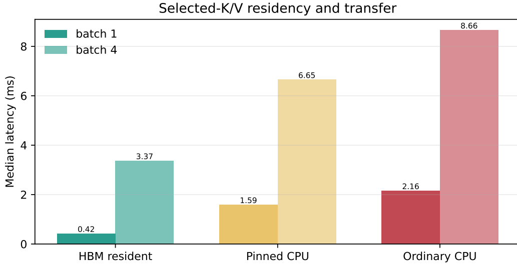
Figure 17: The same logical selection has different physical cost depending on residency. Pinned transfer helps, but does not erase the hierarchy boundary.
