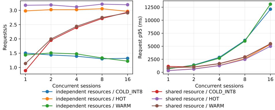
Figure 26: Shared and independent MLX resources through 16 concurrent sessions. The finite waves include promotion and serialized model queueing.
