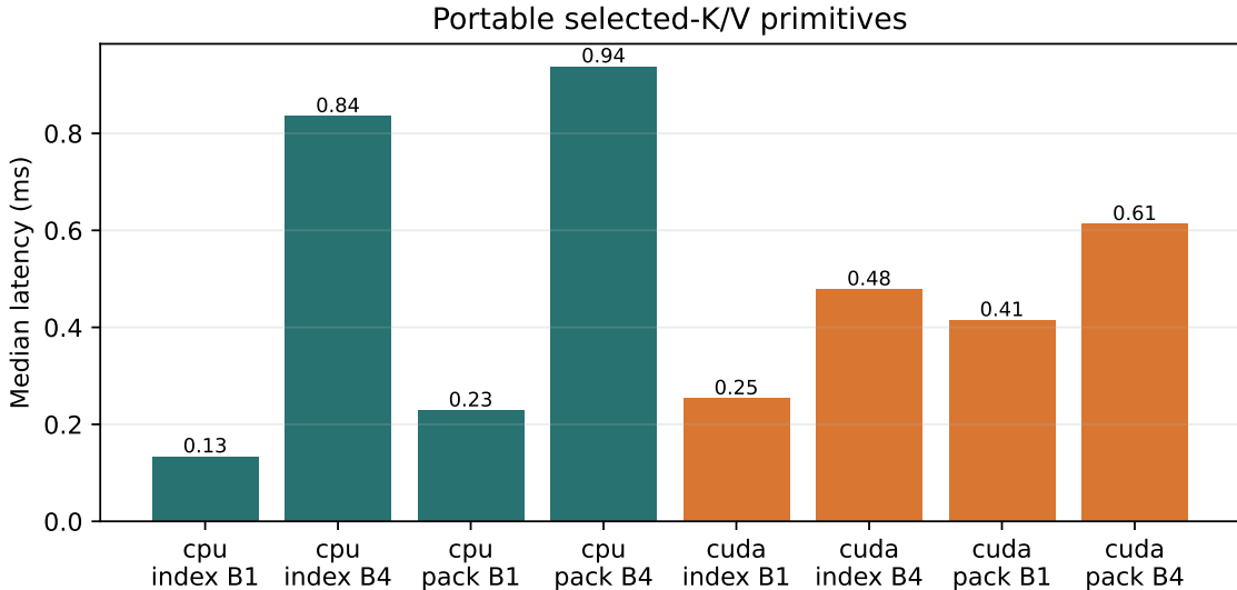
Figure 16: Portable primitive latency. This older GPU does not make small batch-one gathers faster than the CPU, but CUDA scales better at batch four.
