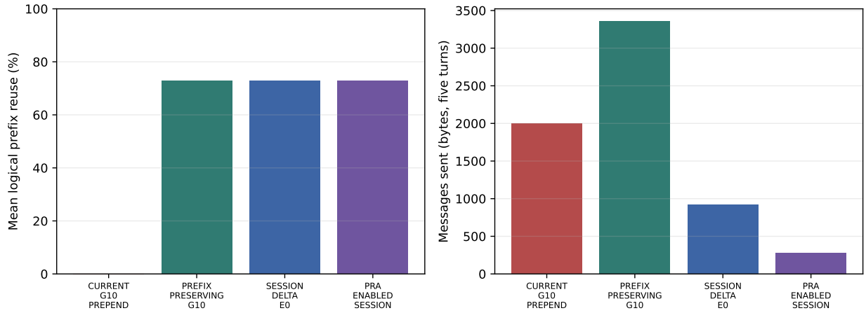
Figure 12: Five-turn deterministic gateway profile. The left panel reports logical reuse of the exact prior serialized message prefix after turn one; the right reports message bytes sent. Resource bytes are reported separately in Table 14.
