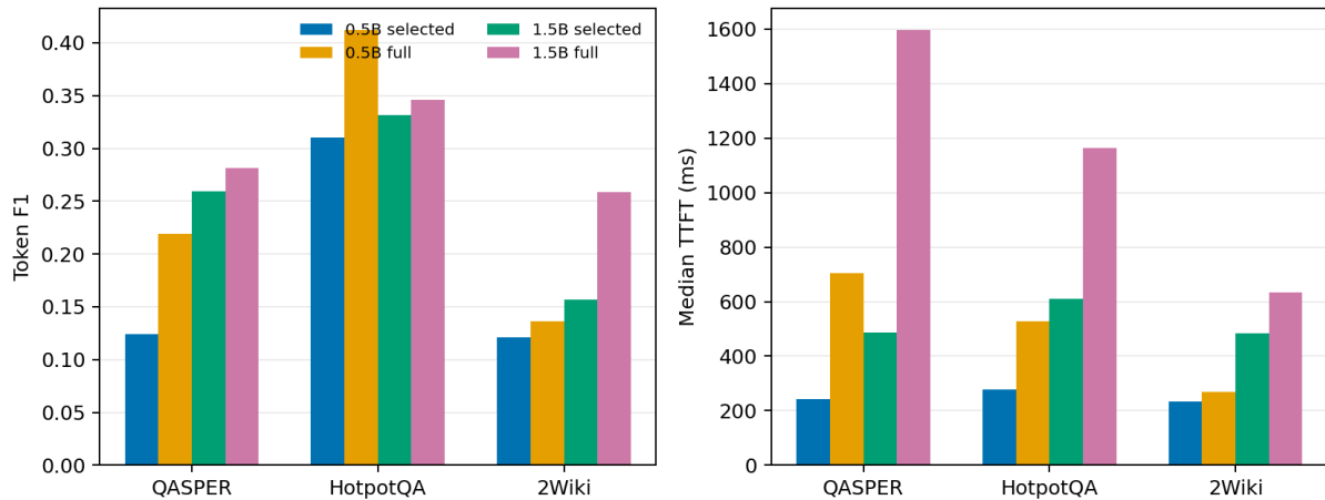
Figure 2: Cross-model quality and TTFT with frozen evidence selection. Scaling the model improves selected-context quality, but does not remove the dataset-specific value of additional context.
