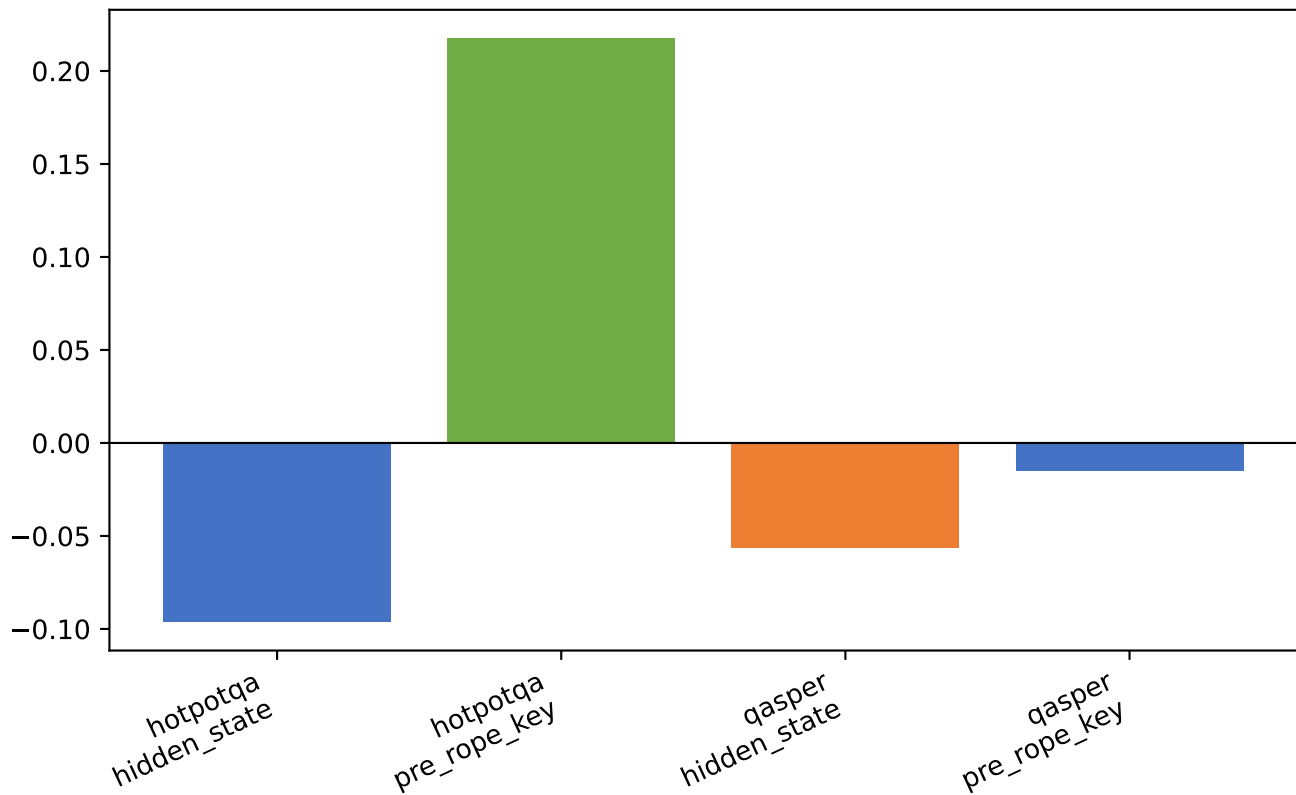
Score-position correlation
