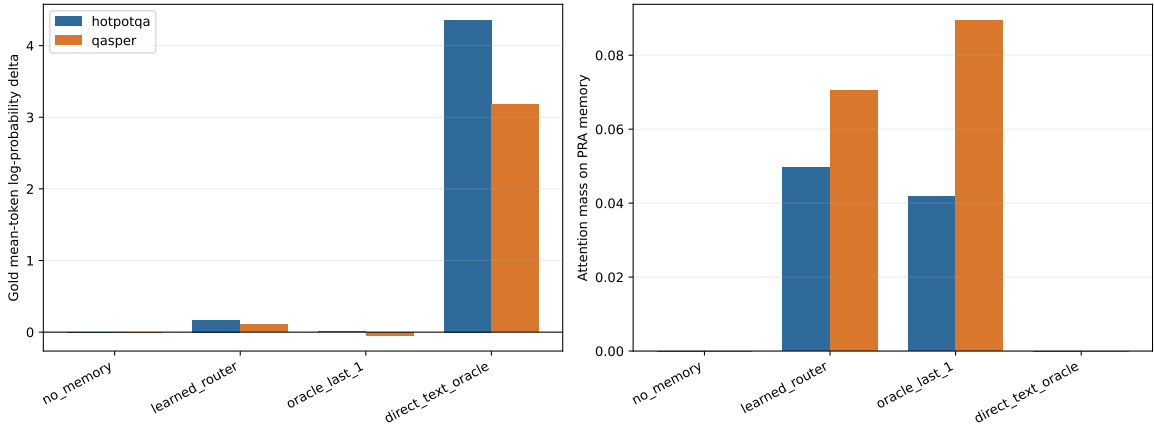
Figure 7: Gemma consumes routed native K/V, but direct text remains much stronger. Gold-token likelihood changes under learned routing, whereas the single-global-layer forced replay is neutral in aggregate. Attention mass confirms that both PRA conditions are active.
