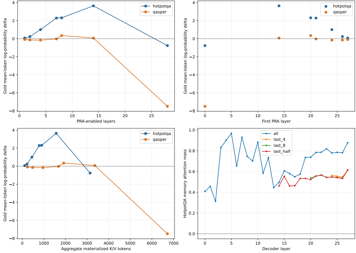
Figure 8: Retrieved native K/V has a depth-dependent causal effect. A contiguous late band approaches the direct-text benefit on HotpotQA, whereas all-layer sparse injection is harmful. The lower panels show that additional exposure also increases materialization cost.
