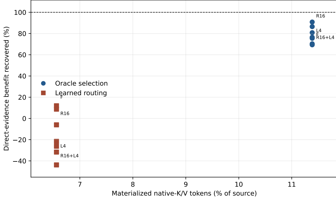
Figure 10: HotpotQA direct-evidence recovery versus physical native-K/V materialization. F, R16, L4, and R16+L4 label the frozen, residual-16, LoRA-4, and combined controls; unlabeled points are the remaining registered widths/ranks. All methods share a fixed memory fraction within a selection mode. Oracle residual 16 raises the ceiling, while every learned adaptation lowers the routed frontier relative to frozen PRA.
