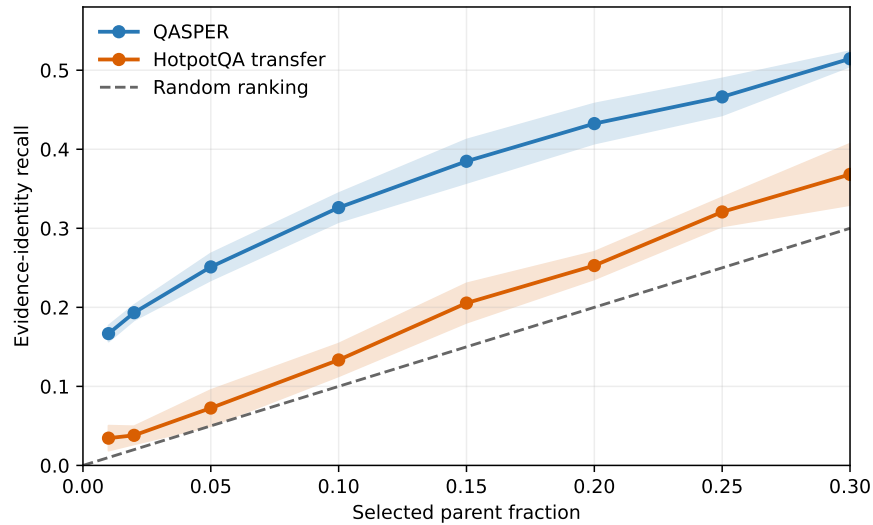
Figure 6: The frozen Gemma router is useful but not high-recall at sparse budgets. Five-seed evidence-identity recall (mean \pm one sample standard deviation) is above random on QASPER, its training domain, and transfers more weakly to HotpotQA. Both domains require exhaustive selection to reach 0.80 identity recall.
