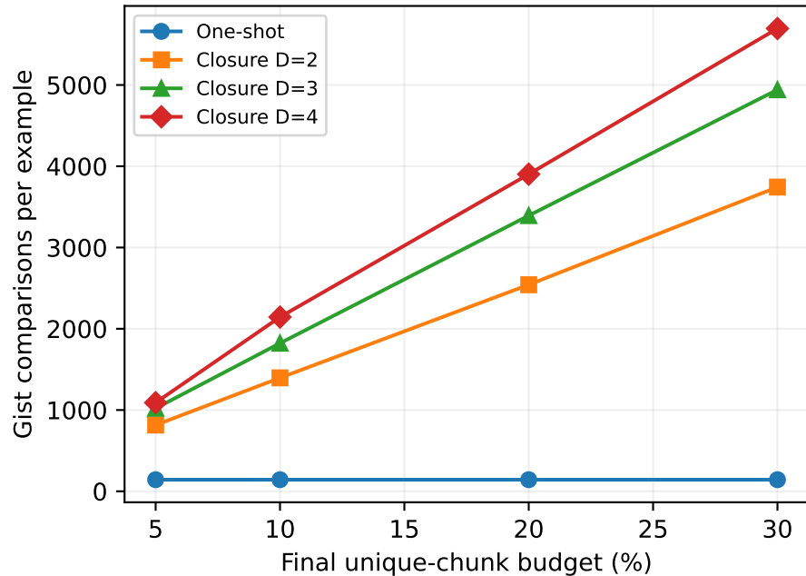
qasper
