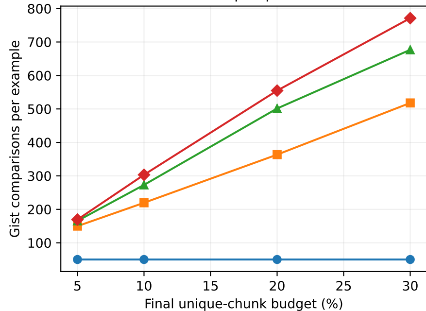
hotpotqa
