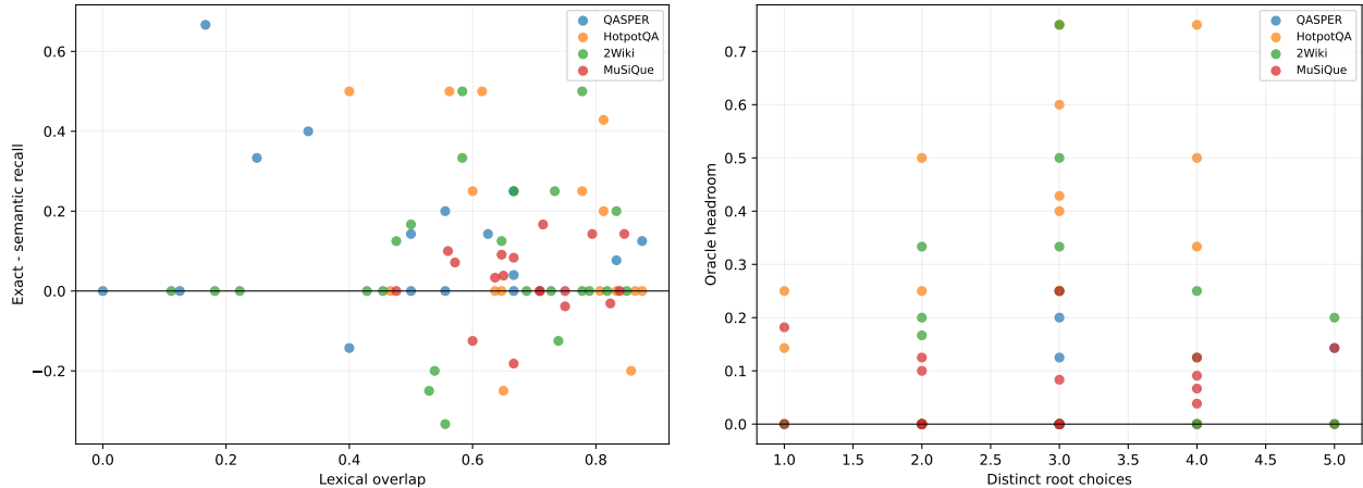
Figure 4: Left: gold query/evidence lexical overlap versus exact-over-gist recall. Right: root-channel disagreement versus validation-fixed channel-oracle headroom. Geometry is explanatory; neither variable is used as gold input to the selector.
