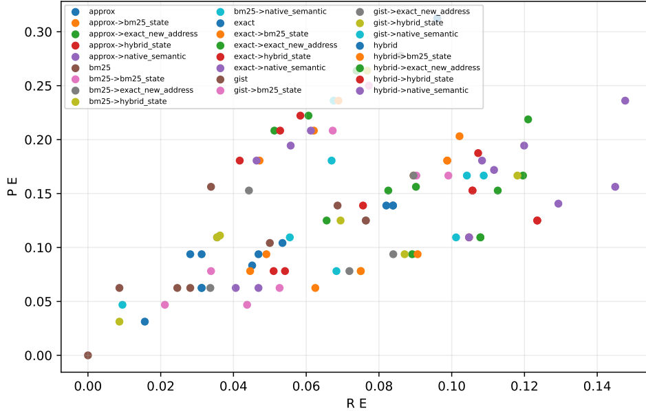
Figure 19: Evidence precision against evidence recall for every held-out root and root–successor policy. The full 25-pair surface is retained rather than only the cohort-wise maxima in Table 4.
