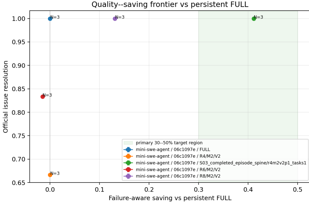
Figure 6: Failure-aware quality-saving frontier for the replacement N=3 cohort. The shaded band is the predeclared 30–50% target; P1 enters it while preserving all paired successes in both executions. Error bars are absent because this cohort contains only one ordered sequence family.
