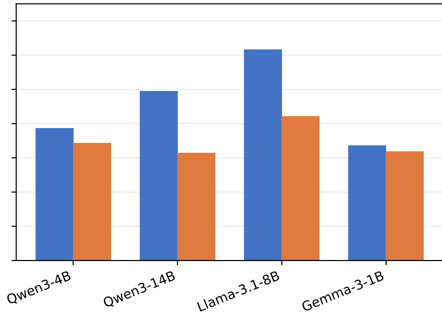
HotpotQA
