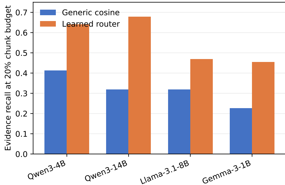
QASPER
