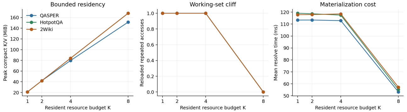
Figure 9: Five-seed compact-K/V pressure over QASPER, HotpotQA, and 2Wiki. Each seed visits eight resources twice and then revisits the first. The budget K = 8 is the first condition that fits the working set.
