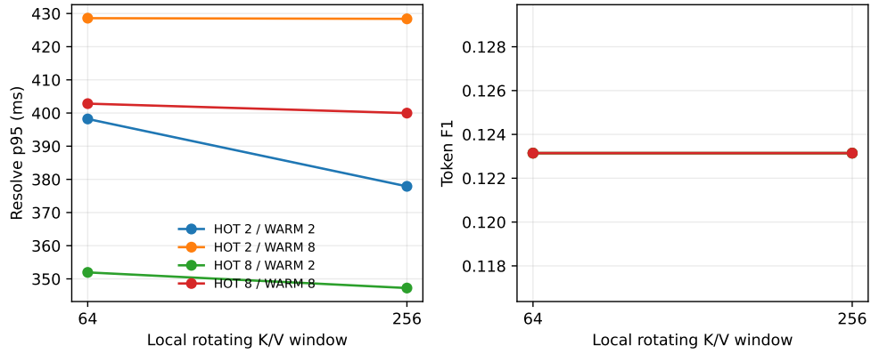
Figure 14: Local-window size has no quality effect in this bounded decode; HOT admission dominates median resolution, while broad WARM retention does not improve the tail on this host.
