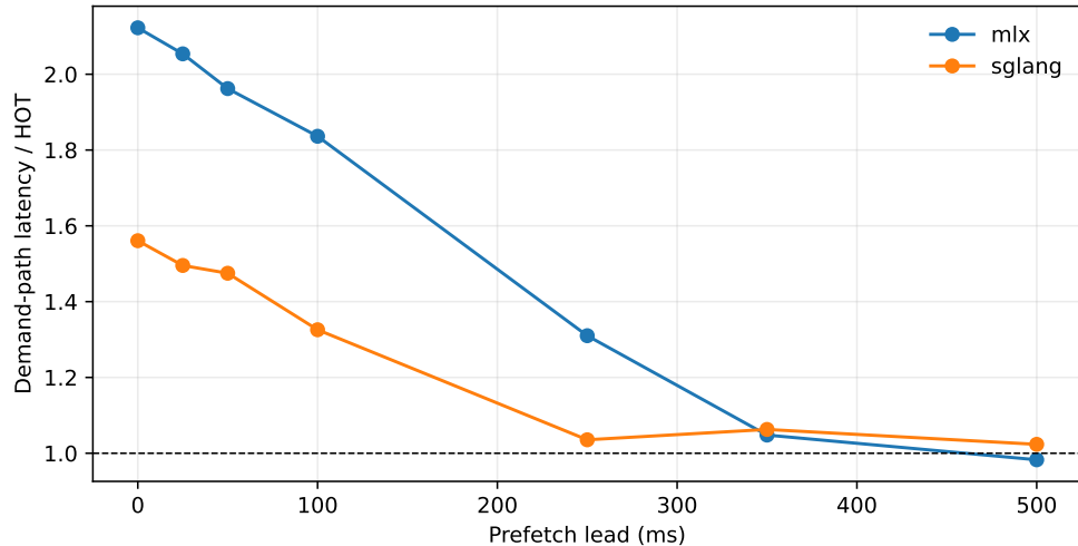
Figure 11: Promotion lead trades demand-path stall for speculative work. The dashed line is HOT request latency.
