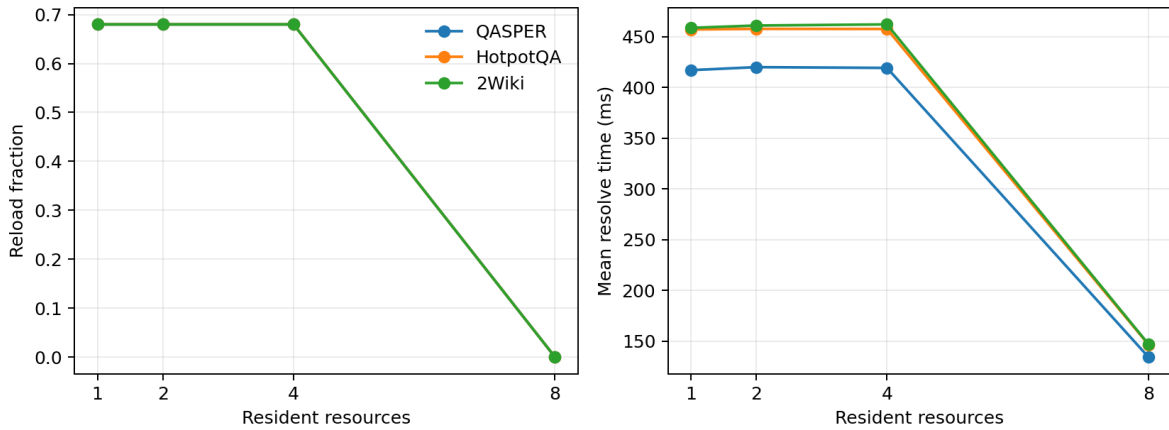
Figure 10: The eight-resource working-set threshold at Qwen3-4B. Fitting the complete set removes repeat reloads and lowers mean resolution; it does not remove each resource’s first cold ingestion.
