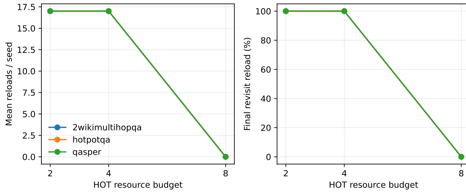
Figure 13: The eight-resource working-set threshold appears consistently across all three datasets.
