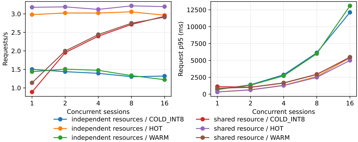
Figure 12: MLX physical-tier concurrency. Shared WARM amortizes one promotion; independent WARM scales storage work with the number of resources.
