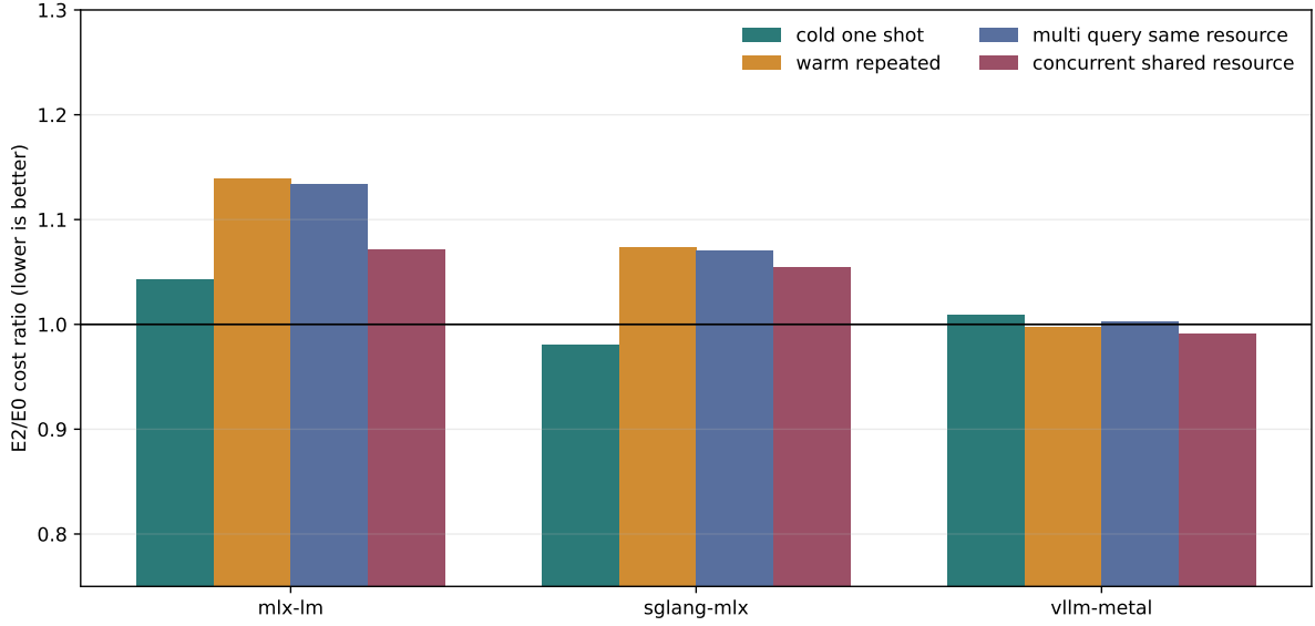
Figure 8: Expanded 149-question representation-cost confirmation across all three engines. Retrieval and selected evidence are held fixed.
