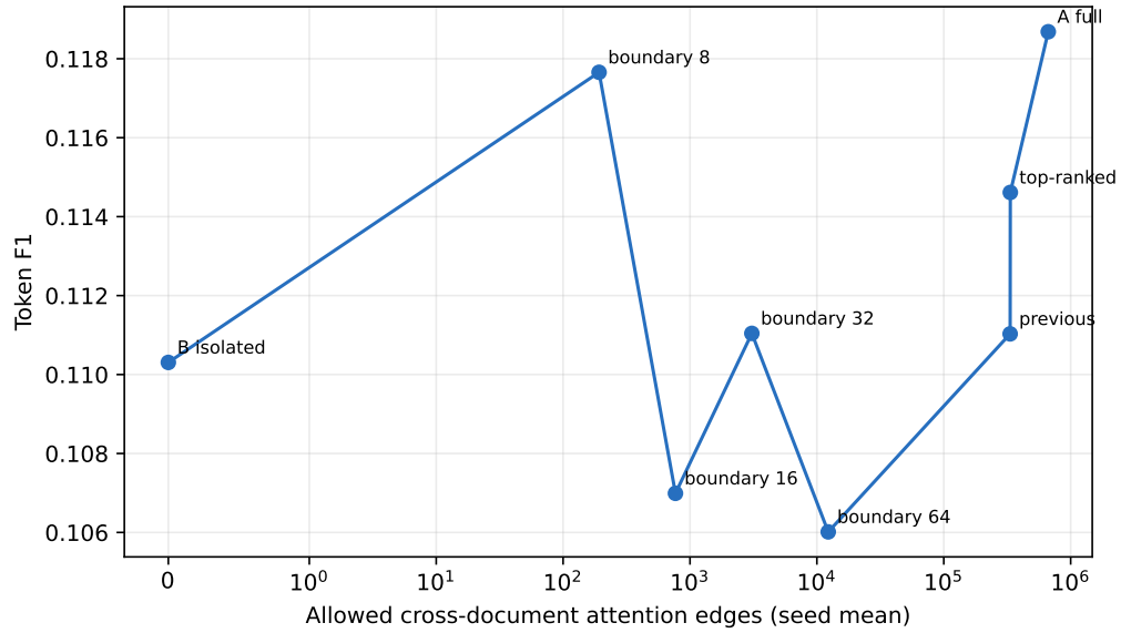
Figure 14: Token F1 against allowed document-to-document attention edges. More interaction is not monotonically better on the measured cohort.
