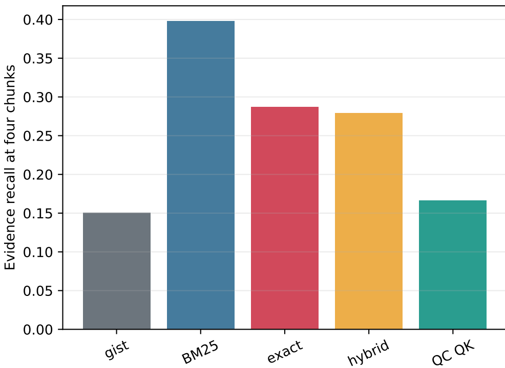
HOTPOTQA
