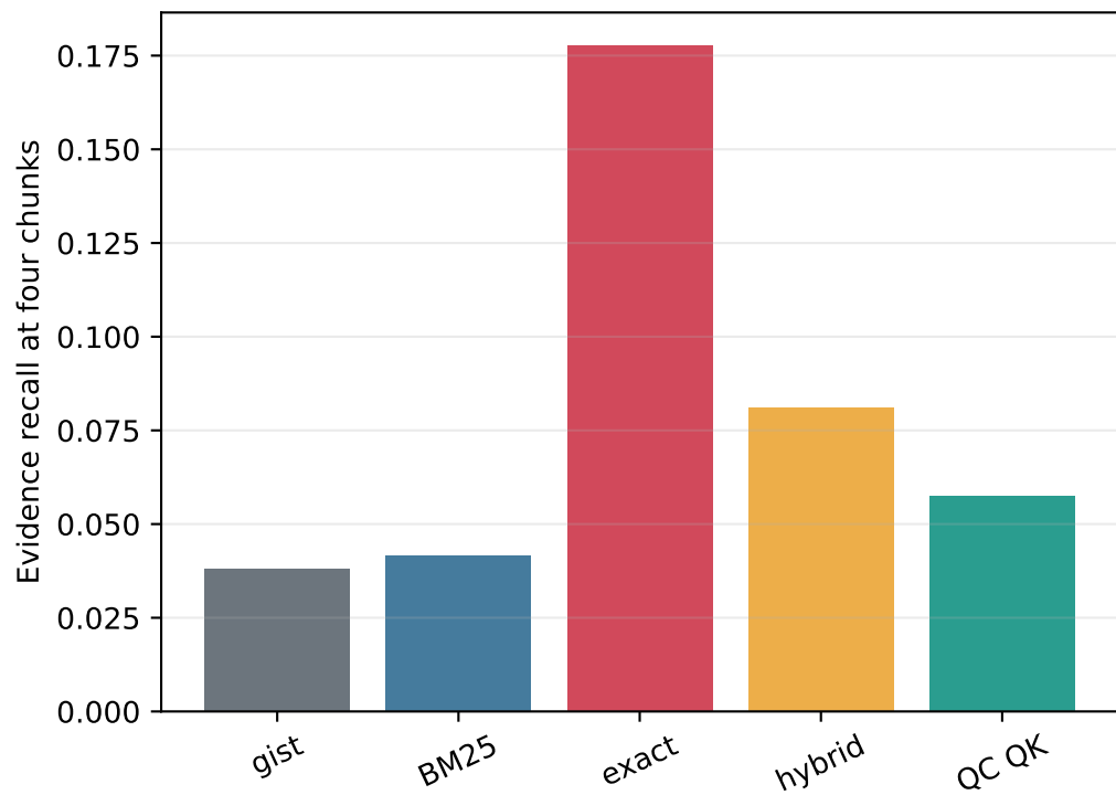
QASPER
