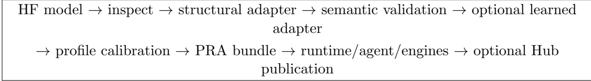
Figure 31: The model-onboarding path. Each arrow is a separately inspectable service boundary rather than an implicit side effect of one CLI callback.
