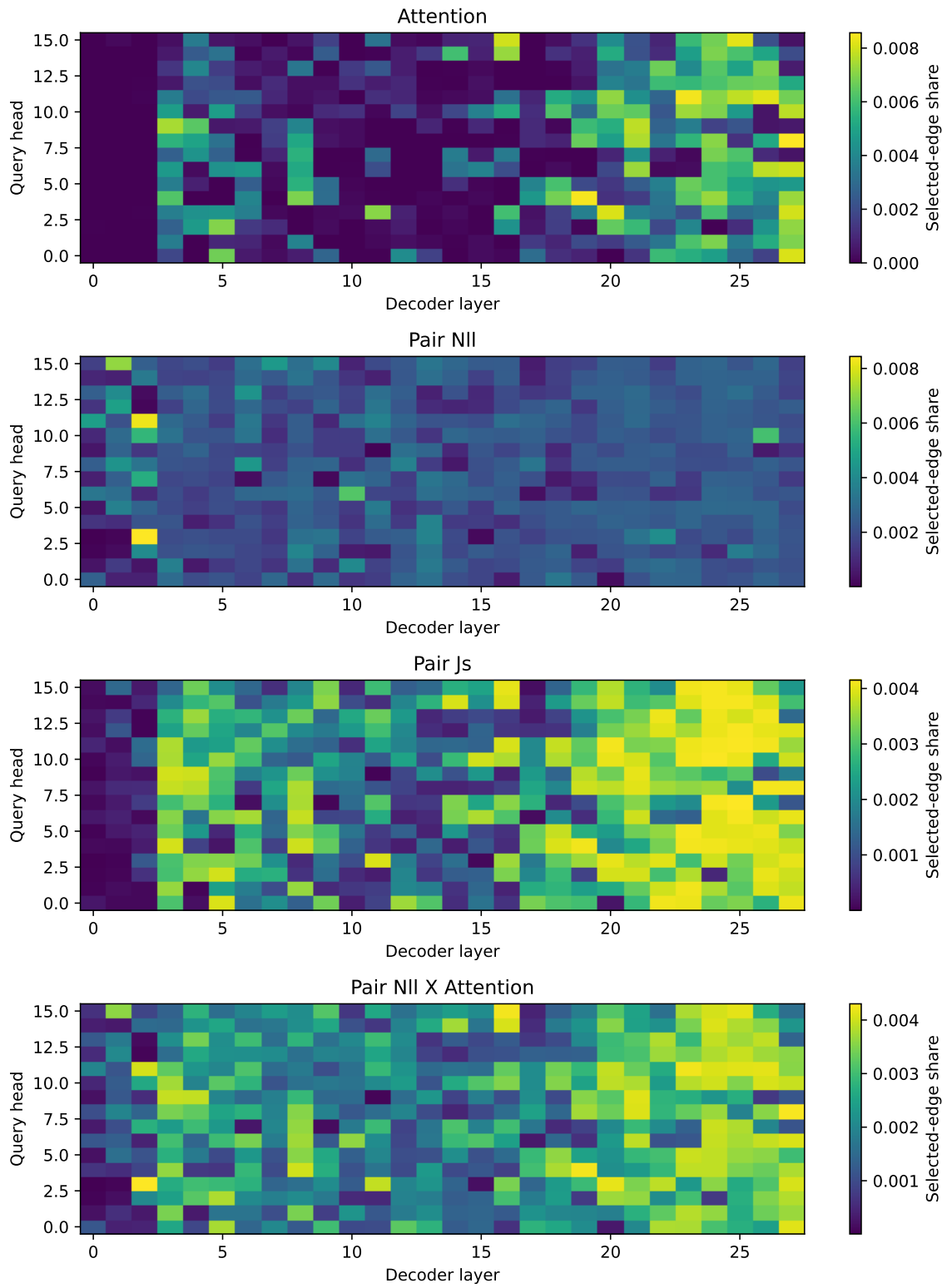
Figure 4: Layer-head allocation of each .1% plan over 150 frozen test questions. Color is selected-edge share within a policy.
