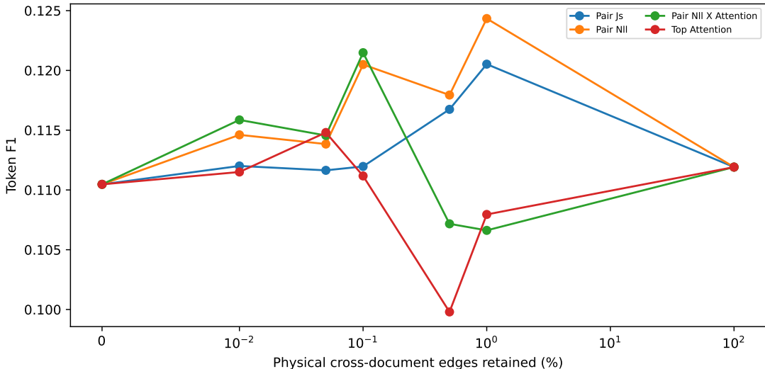
Figure 3: Powered-test F1 frontiers for observational and interventional rankings. Causal pair rankings improve the mean sparse frontier, but all curves remain non-monotonic; lines aid reading and do not imply interpolation.
