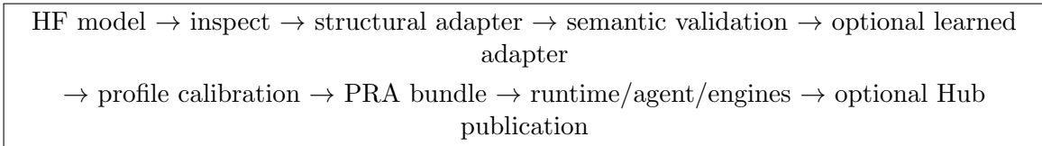
Figure 13: The model-onboarding path. Each arrow is a separately inspectable service boundary rather than an implicit side effect of one CLI callback.
