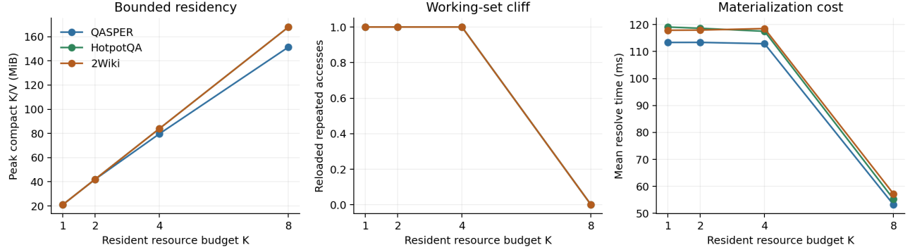
Figure 4: Five-seed compact-K/V pressure over QASPER, HotpotQA, and 2Wiki. Each seed visits eight resources twice and then revisits the first. The budget K = 8 is the first condition that fits the working set.
