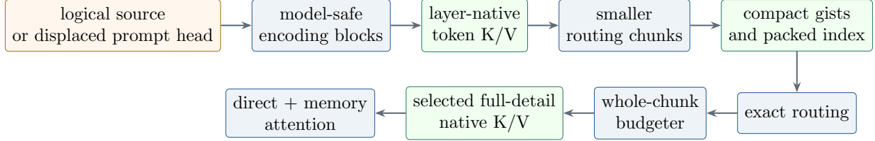
Figure 2: PRA compresses the search representation, not the selected memory payload. Contextual encoding produces native state, compact gists select addresses, and full-detail token K/V enters bounded attention.
