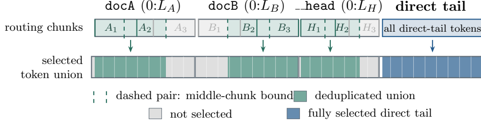
Figure 1: Overlapping chunks and one per-token PRA selection. Each document and the rollover #_head is chunked in its own local coordinate space. Chunk spans share one row and adjacent chunks overlap by approximately 30%; dashed vertical pairs delimit the middle chunks A_2 , B_2 , and H_2 . Every token in a selected chunk is retained. Selected spans are merged into the solid-green union below, so overlapping tokens appear exactly once. The blue direct tail is selected in full, while gray token spans remain addressable but inactive in this attention operation.
