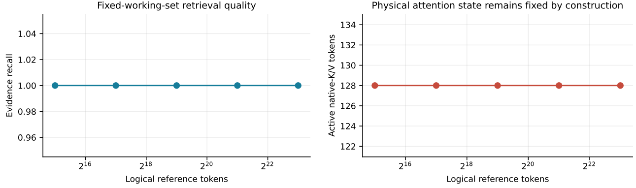
Figure 1: Address-space scaling at fixed task difficulty. Recall remains saturated while selected attention state is constant. Confidence intervals collapse because all five seeds agree; the result should be read with the task-separability caveat.
