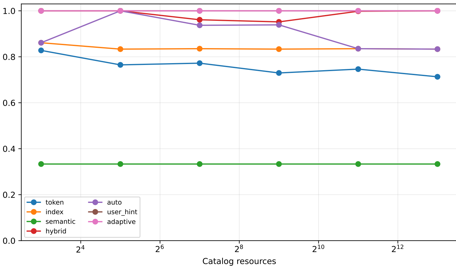
Held-out top-1 selection accuracy
