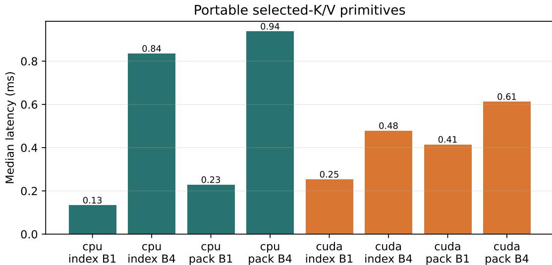
Figure 4: Portable primitive latency. This older GPU does not make small batch-one gathers faster than the CPU, but CUDA scales better at batch four.
