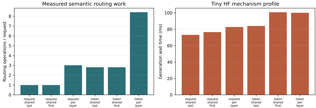
Figure 3: Five-seed tiny-HF mechanism profile. Routing operations validate the execution contract; wall time is host- and model-specific and is not a serving speed claim.
