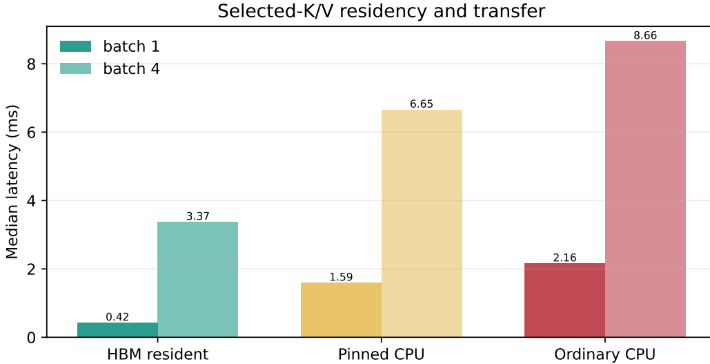
Figure 5: The same logical selection has different physical cost depending on residency. Pinned transfer helps, but does not erase the hierarchy boundary.
