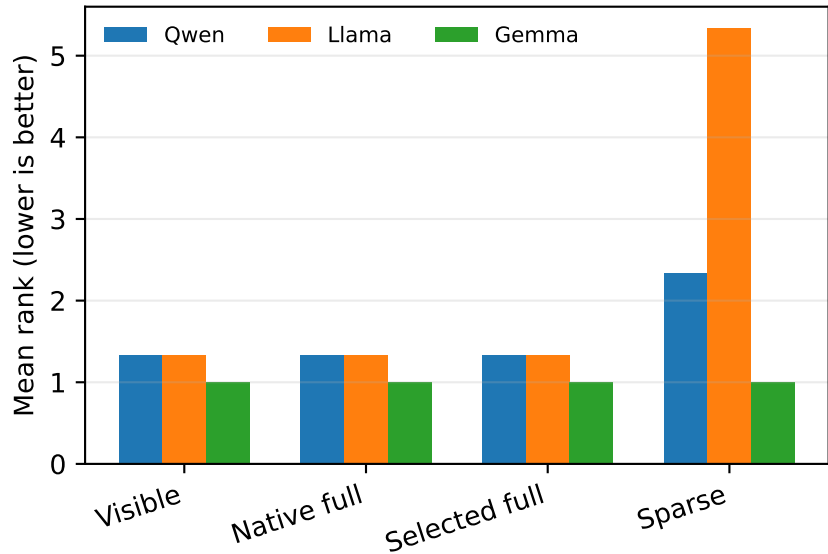
Expected next-token rank
