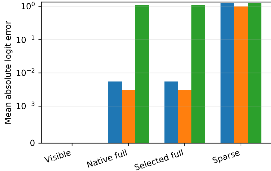
Deviation from visible prefix
