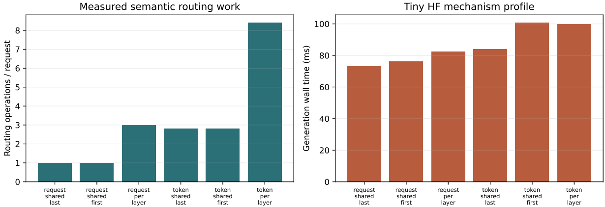
Figure 4: Five-seed tiny-HF mechanism profile. Routing operations validate the execution contract; wall time is host- and model-specific and is not a serving speed claim.
