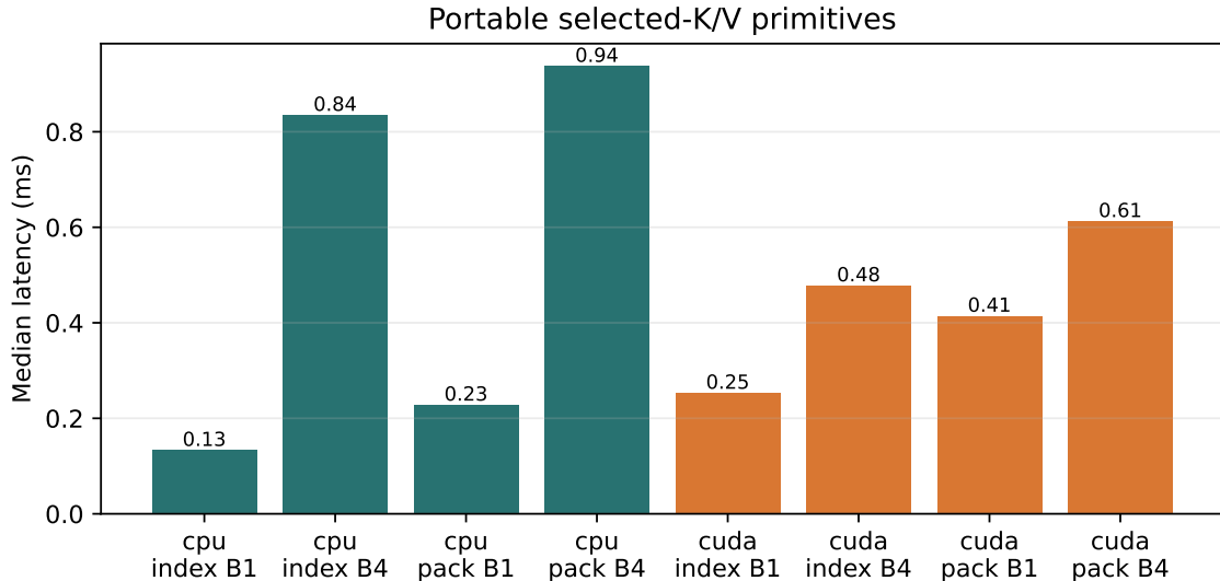
Figure 5: Portable primitive latency. This older GPU does not make small batch-one gathers faster than the CPU, but CUDA scales better at batch four.
